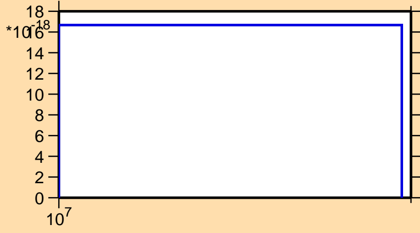
\sigma vs. E for ^{36}\text{Ar}(n,nd)
