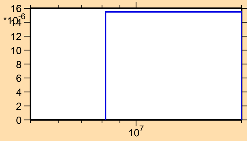
\sigma vs. E for ^{36}\text{Ar}(n,t)
