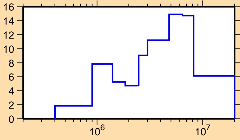
\Delta\sigma/\sigma vs. E for ^{36}\text{Ar}(n,el.)
