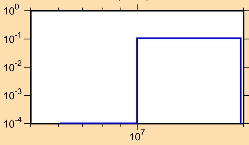
\sigma vs. E for ^{37}\text{Ar}(n,n\alpha)
