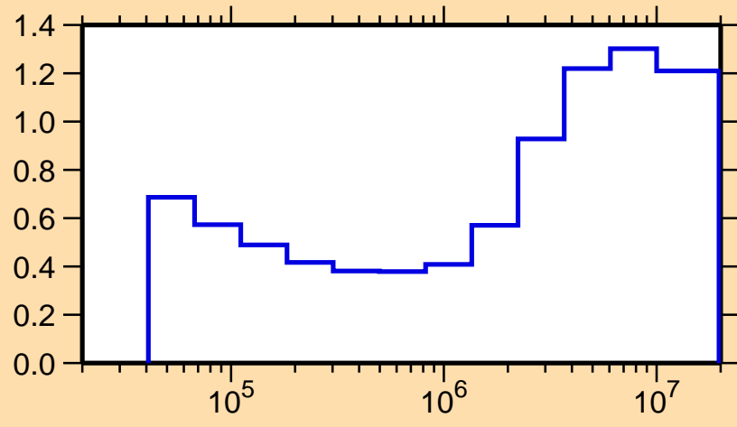
\sigma vs. E for ^{37}\text{Ar}(n,\text{nonel.})
