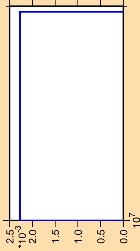
\Delta\sigma/\sigma vs. E for ^{37}\text{Ar} (mt 45)
