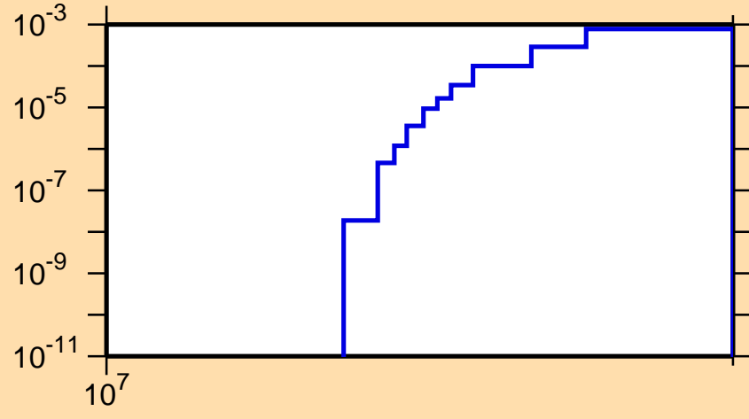
\sigma vs. E for ^{38}\text{Ar}(n,t)
