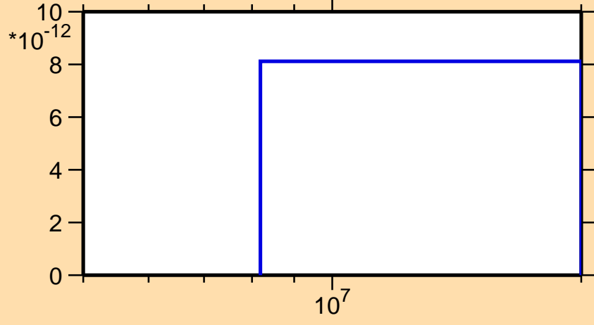
\sigma vs. E for ^{40}\text{Ar}(n,\text{nd})
