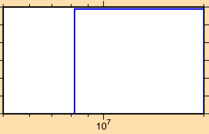
\sigma vs. E for ^{40}\text{Ar}(n,t)
