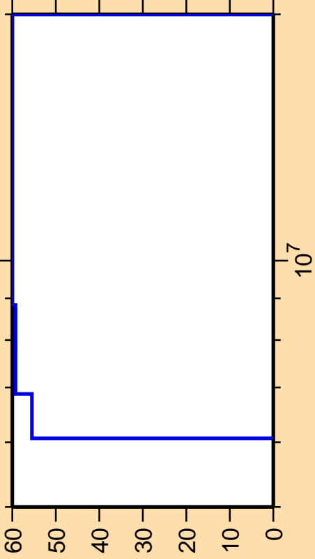
\Delta\sigma/\sigma vs. E for ^{41}\text{Ar}(n,\alpha)
