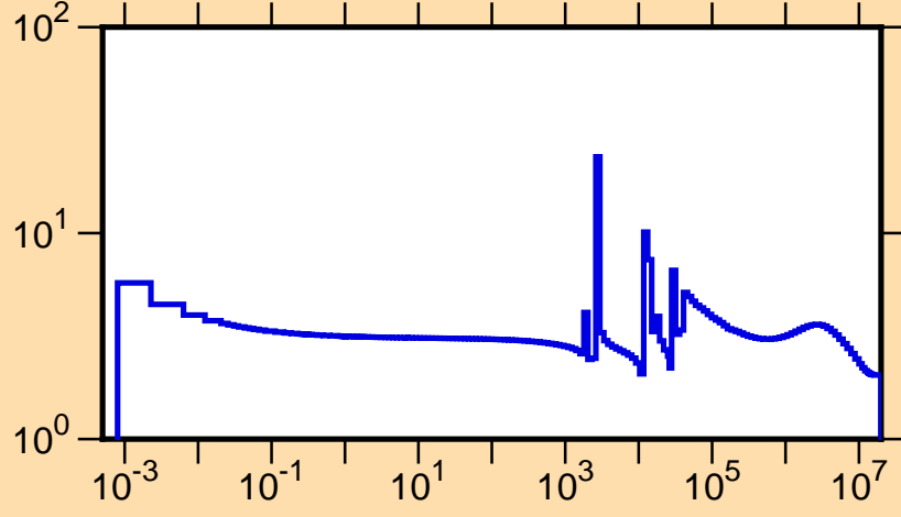
\sigma vs. E for ^{41}\text{Ar}(n,\text{tot.})
