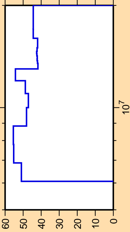
\Delta\sigma/\sigma vs. E for ^{41}\text{Ar}(n,n_1)
