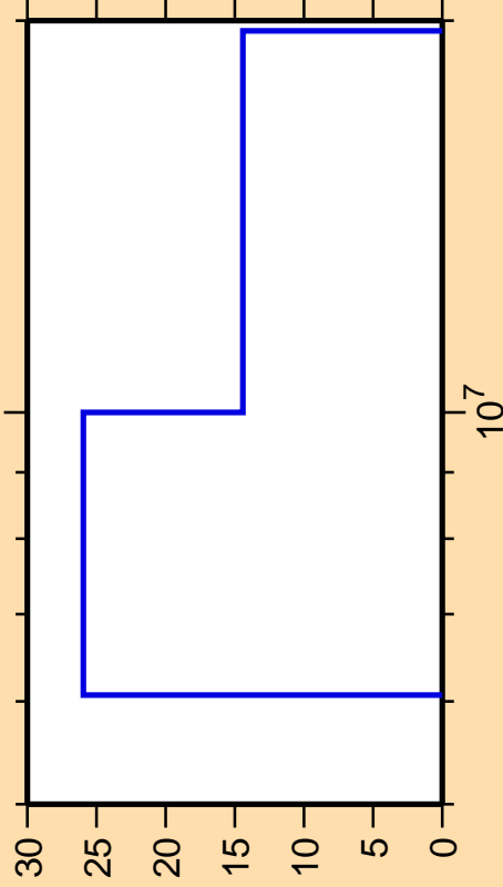
\Delta\sigma/\sigma vs. E for ^{41}\text{Ar}(n,2n)
