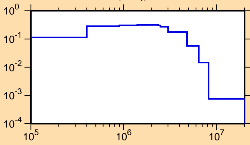
\sigma vs. E for ^{41}\text{Ar}(n,n_1)
