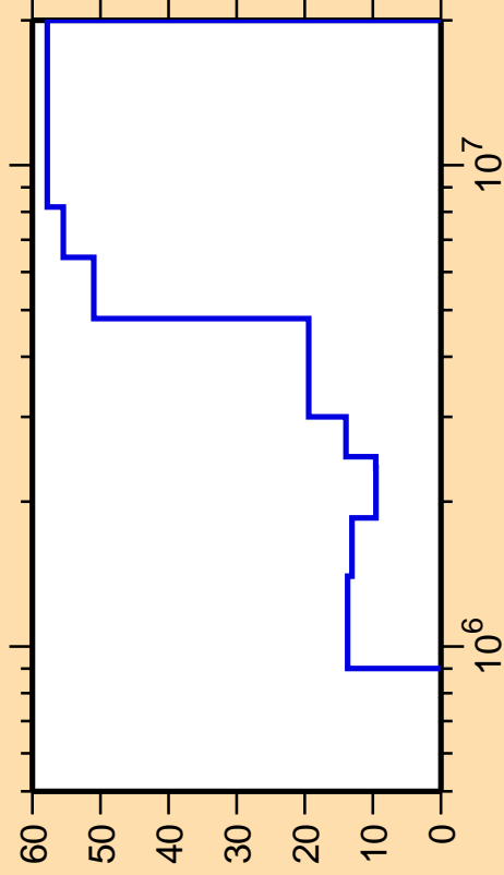
\Delta\sigma/\sigma vs. E for ^{41}\text{Ar}(n,n_3)
