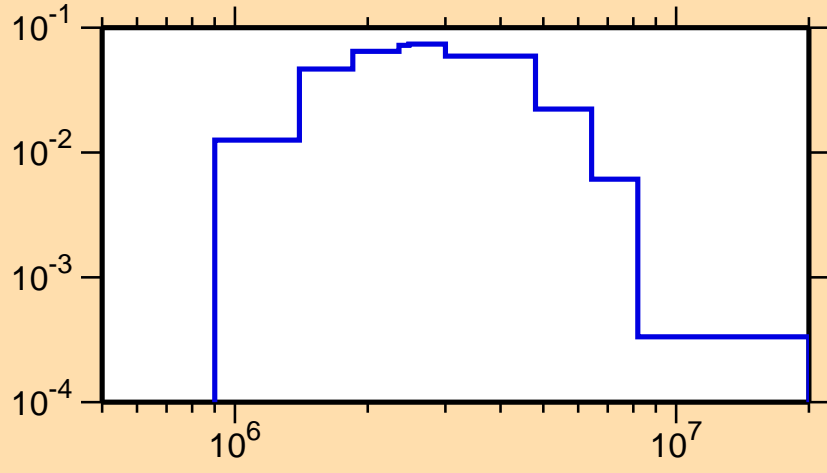
\sigma vs. E for ^{41}\text{Ar}(n,n_3)
