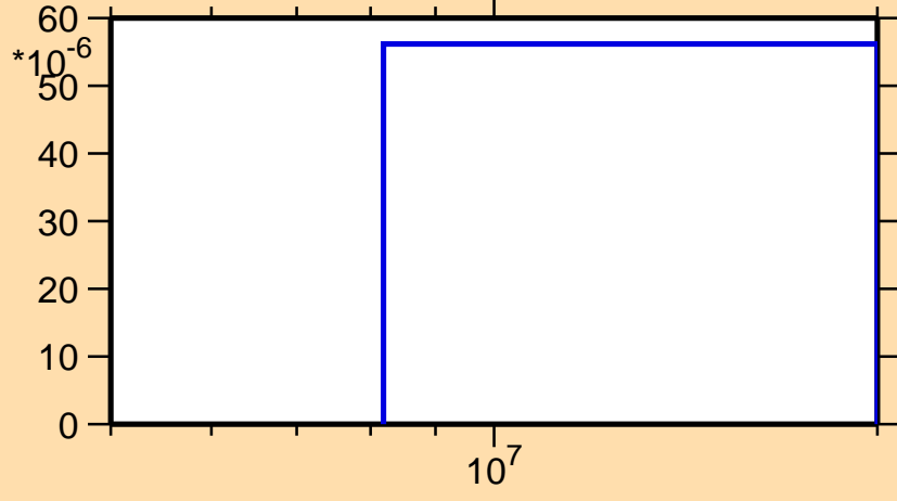
\sigma vs. E for ^{41}\text{Ar}(n,t)
