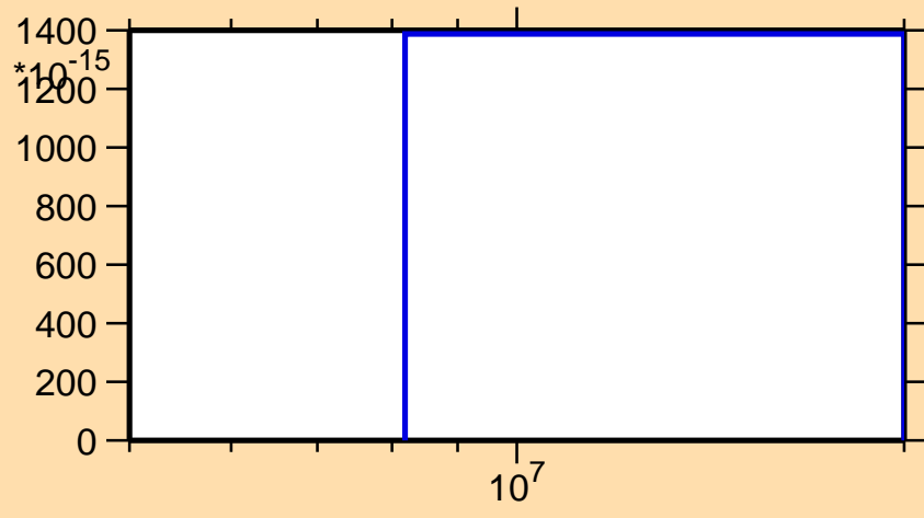
\sigma vs. E for ^{41}\text{Ar}(n,2np)
