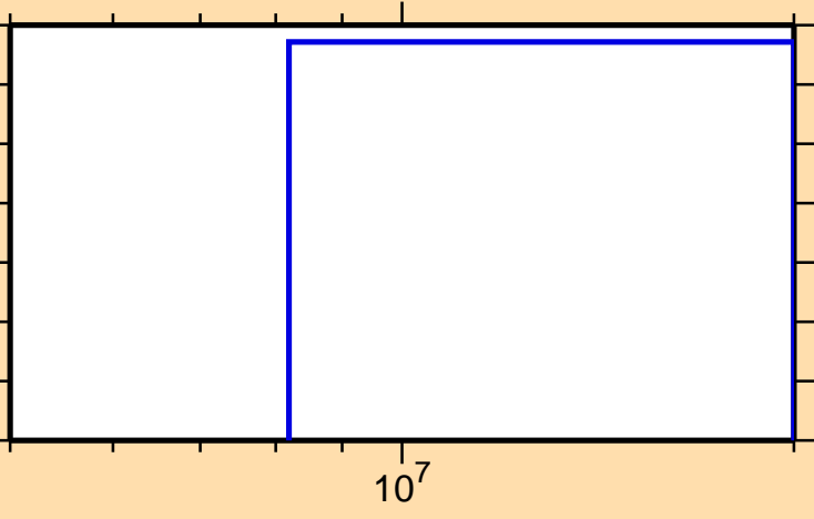
\sigma vs. E for ^{41}\text{Ar}(n,\text{nd})
