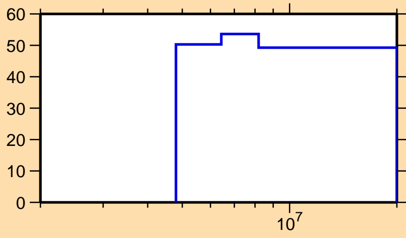
\Delta\sigma/\sigma vs. E for ^{41}\text{Ar}(n,n_1)
