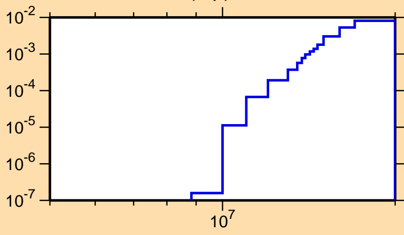
\sigma vs. E for ^{42}\text{Ar}(n,p)
