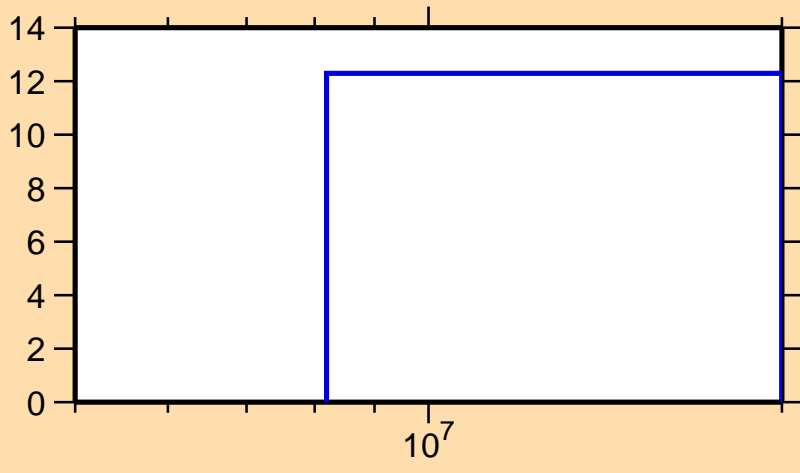
\Delta\sigma/\sigma vs. E for ^{42}\text{Ar}(n,2n)
