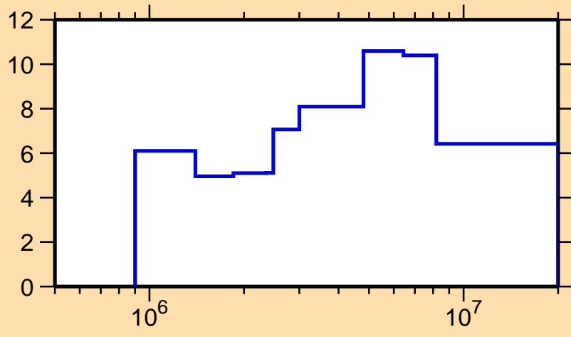
\Delta\sigma/\sigma vs. E for ^{42}\text{Ar}(n,\text{tot.})
