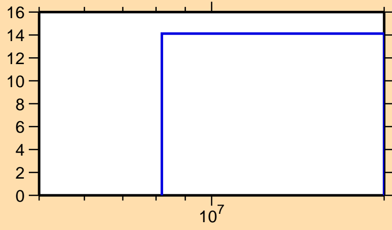
\Delta\sigma/\sigma vs. E for ^{42}\text{Ar}(n,\text{el.})
