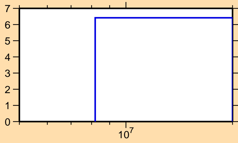
\Delta\sigma/\sigma vs. E for ^{42}\text{Ar}(n,\text{tot.})
