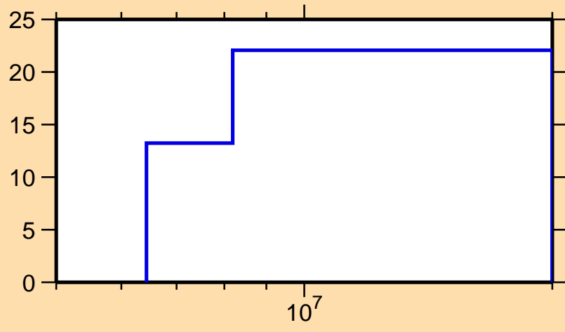
\Delta\sigma/\sigma vs. E for ^{42}\text{Ar}(n,n\text{cont.})
