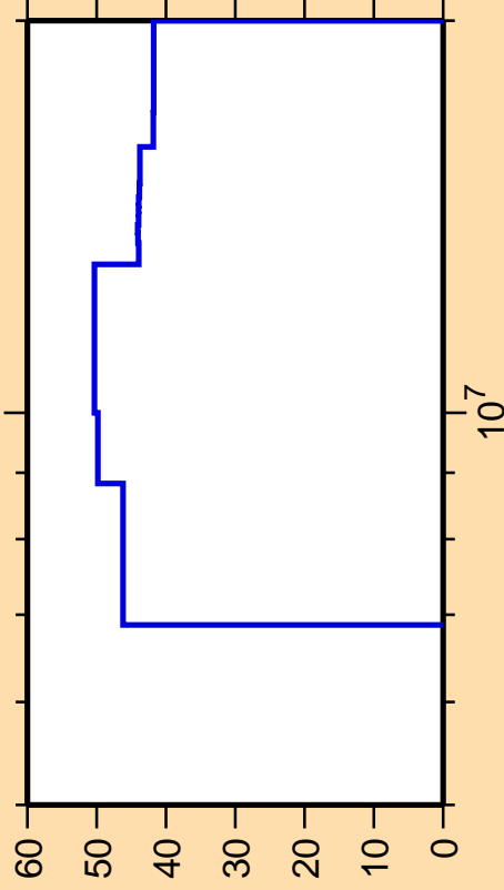
\Delta\sigma/\sigma vs. E for ^{43}\text{Ar}(n,p)
