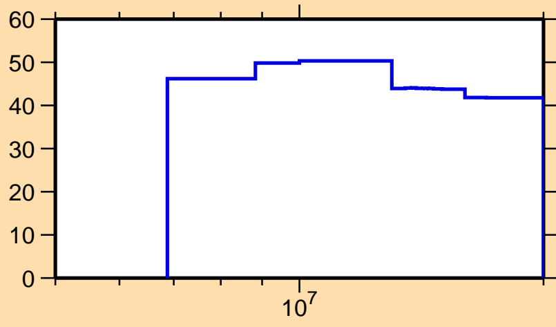
\Delta\sigma/\sigma vs. E for ^{43}\text{Ar}(n,p)
