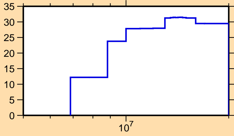
\Delta\sigma/\sigma vs. E for ^{43}\text{Ar}(n,ncont.)
