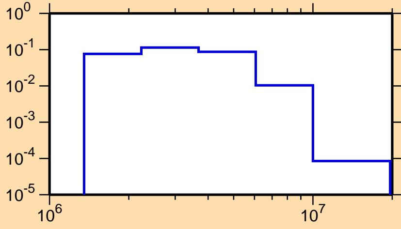
\sigma vs. E for ^{43}\text{Ar}(n,n_2)
