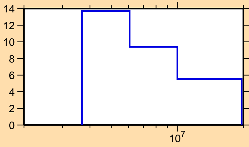
\Delta\sigma/\sigma vs. E for ^{43}\text{Ar}(n,2n)
