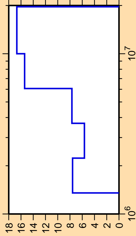
\Delta\sigma/\sigma vs. E for ^{43}\text{Ar}(n,n_2)
