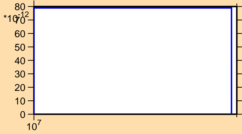
\sigma vs. E for ^{43}\text{Ar}(n,\text{nd})
