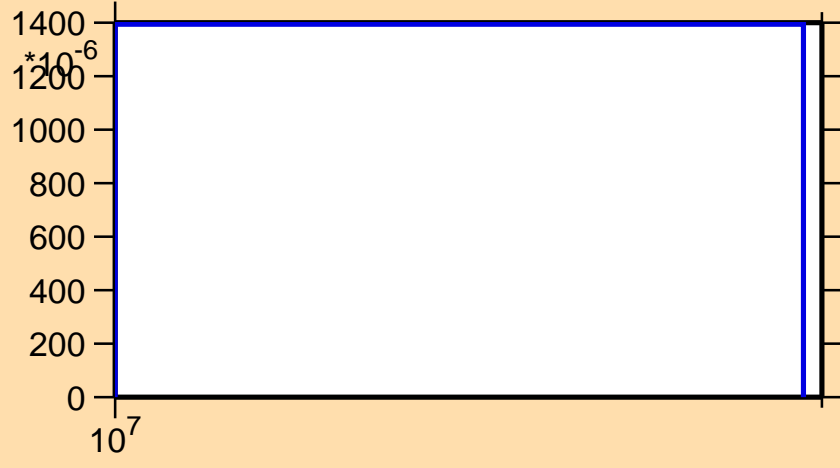
\sigma vs. E for ^{43}\text{Ar}(n,3n)
