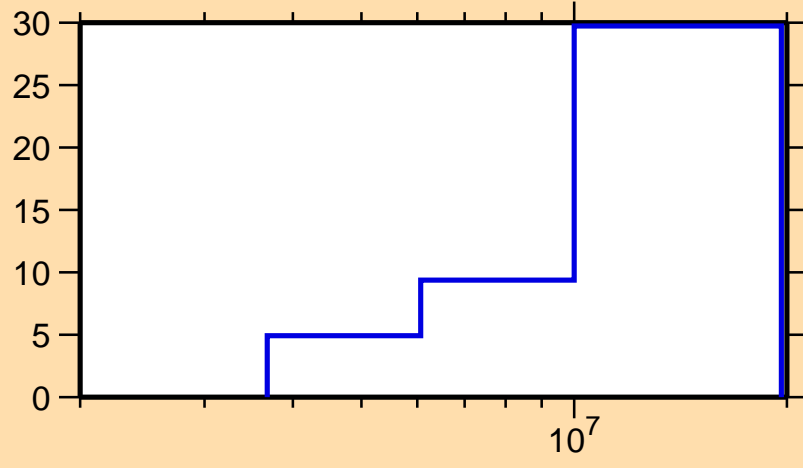
\Delta\sigma/\sigma vs. E for ^{43}\text{Ar}(n,n\text{cont.})
