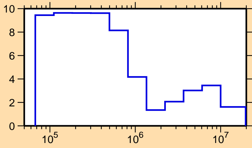
\Delta\sigma/\sigma vs. E for ^{43}\text{Ar}(n,\text{tot.})
