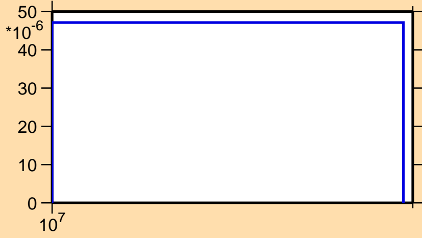
\sigma vs. E for ^{43}\text{Ar}(n,d)
