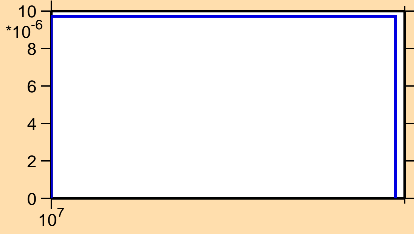
\sigma vs. E for ^{43}\text{Ar}(n,n\alpha)
