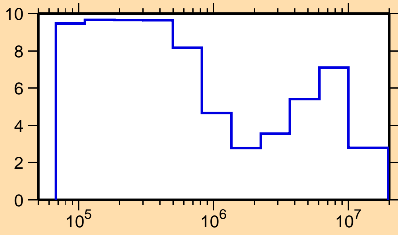
\Delta\sigma/\sigma vs. E for ^{43}\text{Ar}(n,\text{el.})
