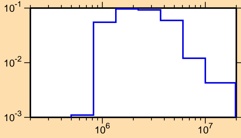
\sigma vs. E for ^{43}\text{Ar}(n,n_1)
