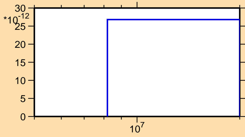
\sigma vs. E for ^{43}\text{Ar}(n,2n\alpha)
