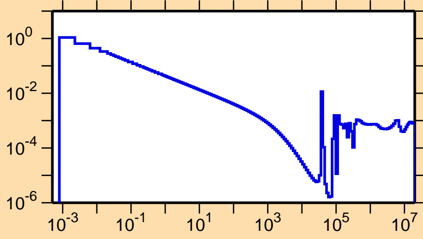
\sigma vs. E for ^{45}\text{Ar}(n,\gamma)
