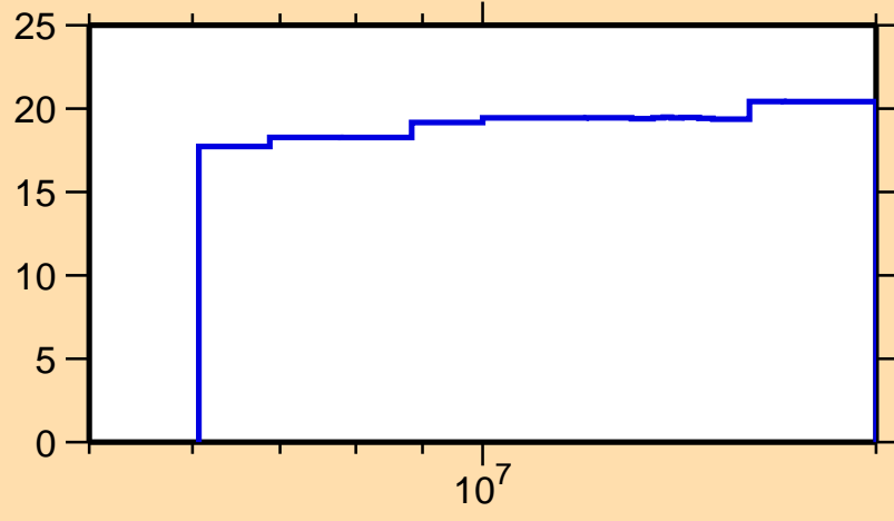
\Delta\sigma/\sigma vs. E for ^{45}\text{Ar}(n,n\text{onel.})
