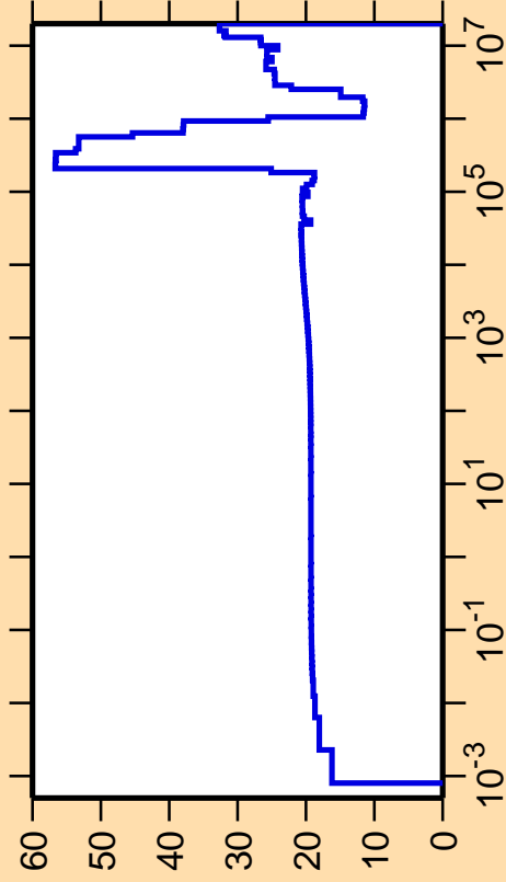
\Delta\sigma/\sigma vs. E for ^{45}\text{Ar}(n,\text{el.})
