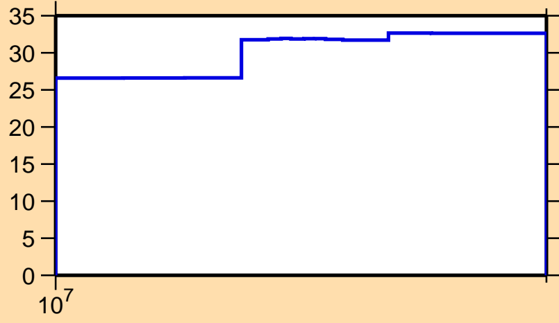
\Delta\sigma/\sigma vs. E for ^{45}\text{Ar}(n,el.)
