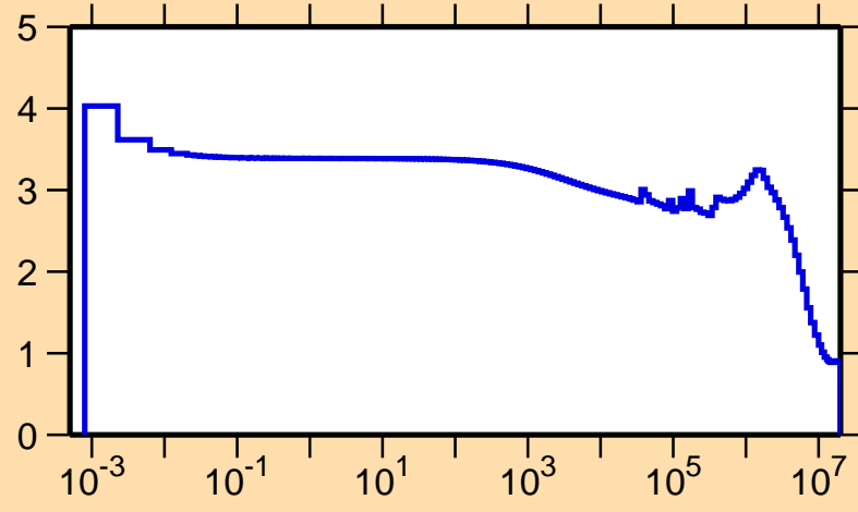
\sigma vs. E for ^{45}\text{Ar}(n,\text{el.})
