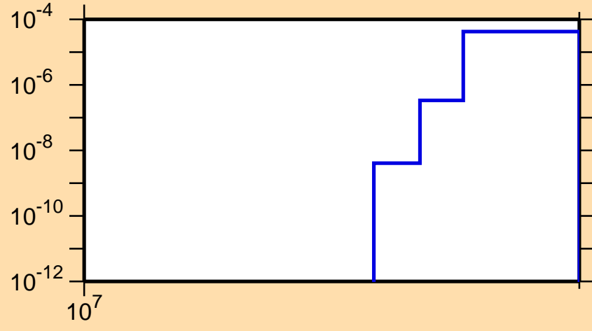
\sigma vs. E for ^{45}\text{Ar}(n,d)
