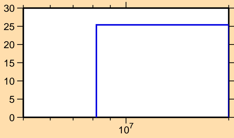
\Delta\sigma/\sigma vs. E for ^{45}\text{Ar}(n,el.)
