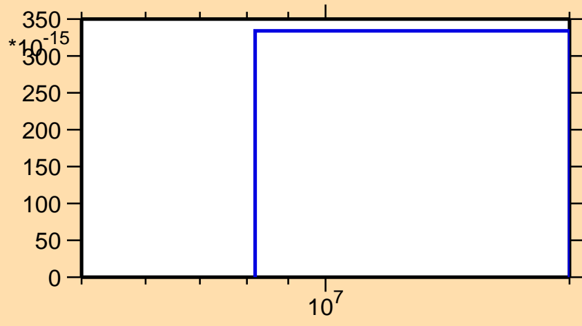
\sigma vs. E for ^{45}\text{Ar}(n,nd)
