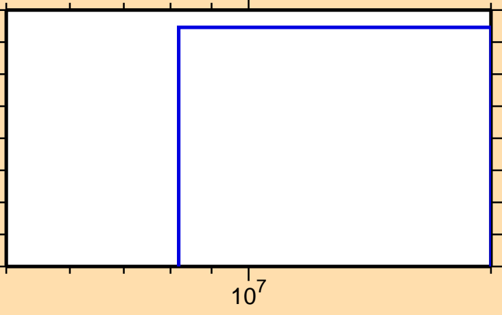
\sigma vs. E for ^{45}\text{Ar}(n,3n)
