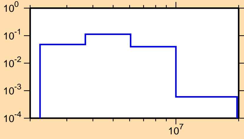
\sigma vs. E for ^{46}\text{Ar}(n,n_4)
