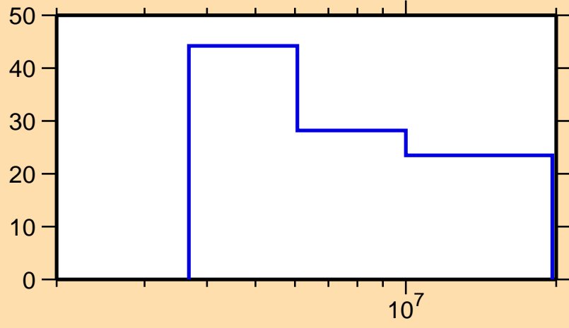
\Delta\sigma/\sigma vs. E for ^{46}\text{Ar}(n,el.)
