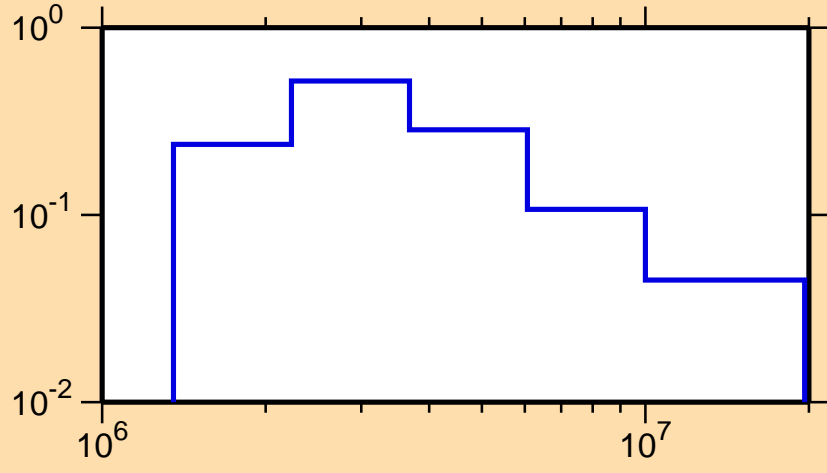
\sigma vs. E for ^{46}\text{Ar}(n,n_1)
