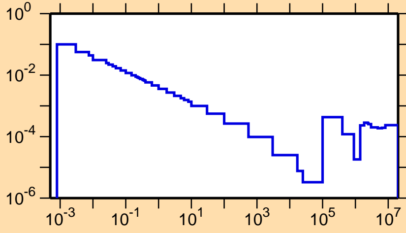
\sigma vs. E for ^{46}\text{Ar}(n,\gamma)
