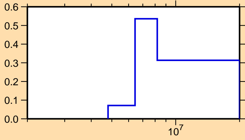
\sigma vs. E for ^{46}\text{Ar}(n,n\text{cont.})
