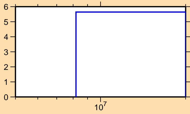
\Delta\sigma/\sigma vs. E for ^{46}\text{Ar}(n,\text{nonel.})
