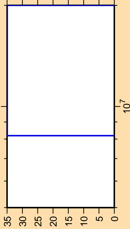
\Delta\sigma/\sigma vs. E for ^{46}\text{Ar}(n,2n)
