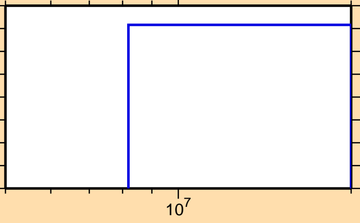
\sigma vs. E for ^{46}\text{Ar}(n,3n)
