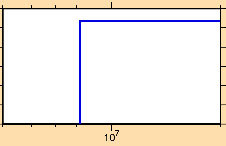
\sigma vs. E for ^{46}\text{Ar}(n,\alpha)
