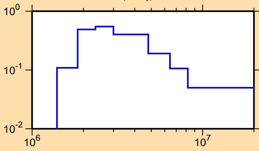
\sigma vs. E for ^{46}\text{Ar}(n,n_1)
