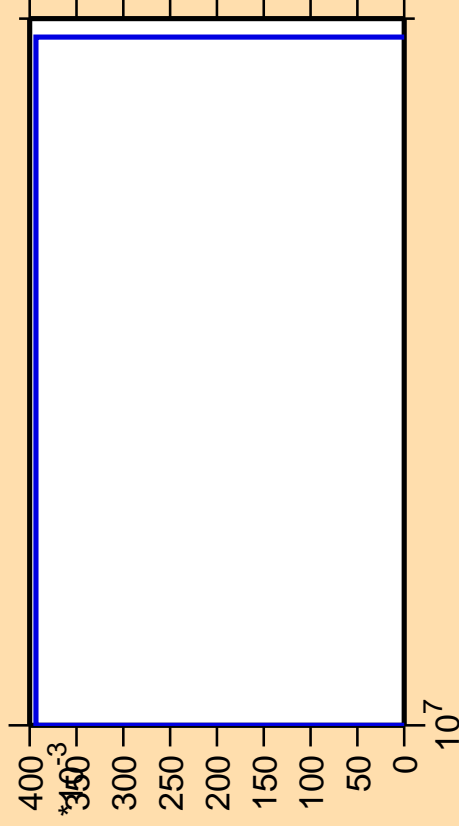
\Delta\sigma/\sigma vs. E for ^{47}\text{Ar}(n,np)
