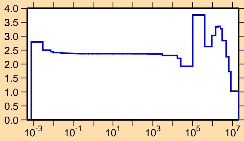
\sigma vs. E for ^{47}\text{Ar}(n,\text{el.})
