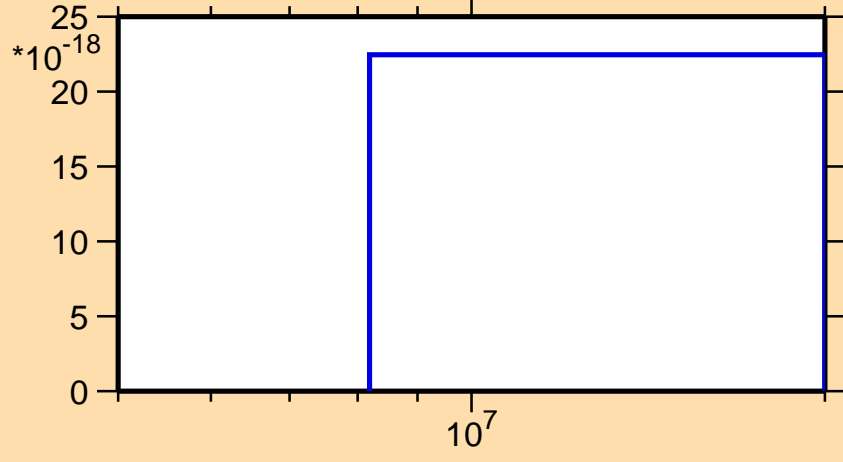
\sigma vs. E for ^{47}\text{Ar}(n,nt)
