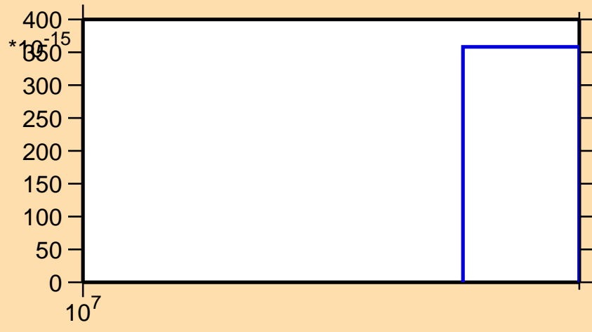
\sigma vs. E for ^{67}\text{As}(n,nt)
