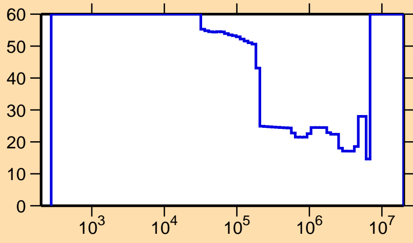
\Delta\sigma/\sigma vs. E for ^{67}\text{As}(n,p)
