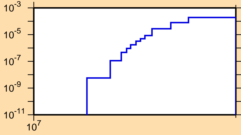
\sigma vs. E for ^{68}\text{As}(n,nd)
