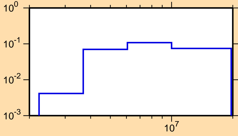
\sigma vs. E for ^{68}\text{As}(n,n\text{cont.})
