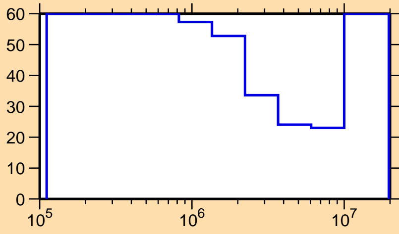
\Delta\sigma/\sigma vs. E for ^{68}\text{As}(n,n_1)
