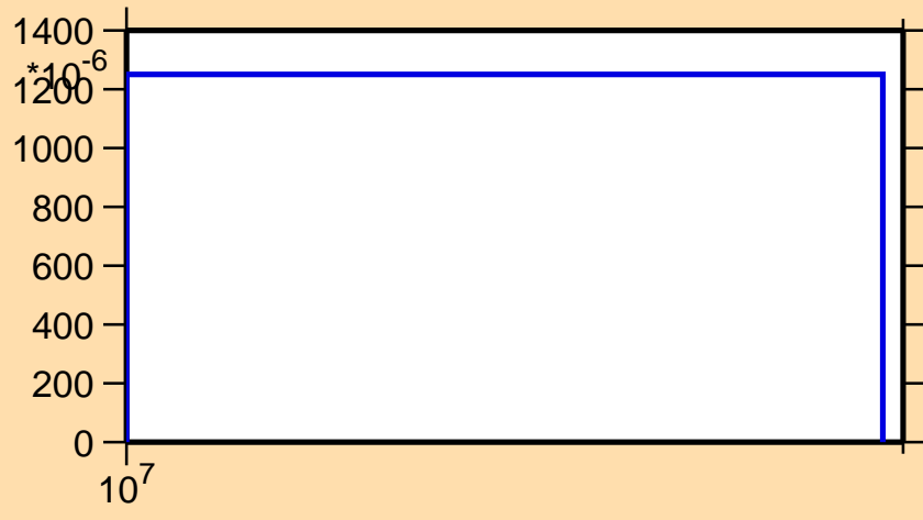
\sigma vs. E for ^{68}\text{As}(n,2n)
