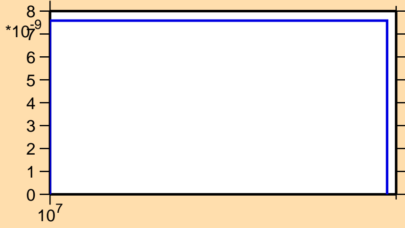
\sigma vs. E for ^{68}\text{As} (mt 34)
