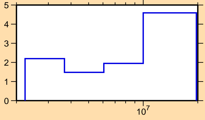
\Delta\sigma/\sigma vs. E for ^{68}\text{As}(n,\text{tot.})
