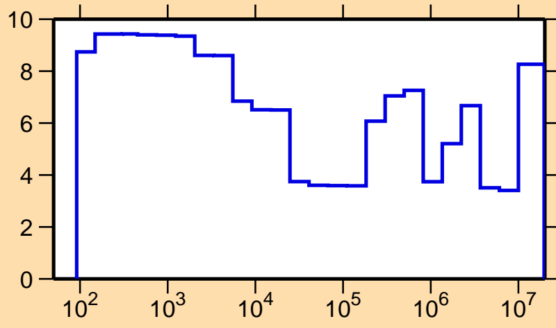
\Delta\sigma/\sigma vs. E for ^{68}\text{As}(n,el.)
