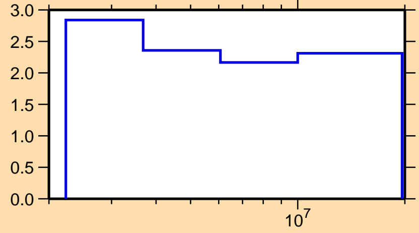
\Delta\sigma/\sigma vs. E for ^{68}\text{As}(n,\text{nonel.})
