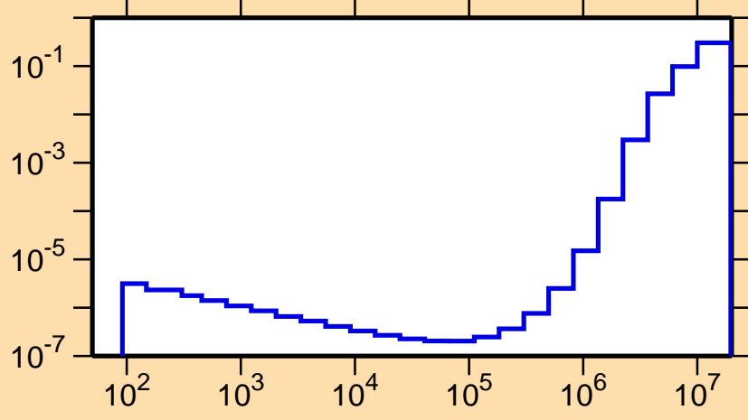
\sigma vs. E for ^{68}\text{As}(n,p\alpha)
