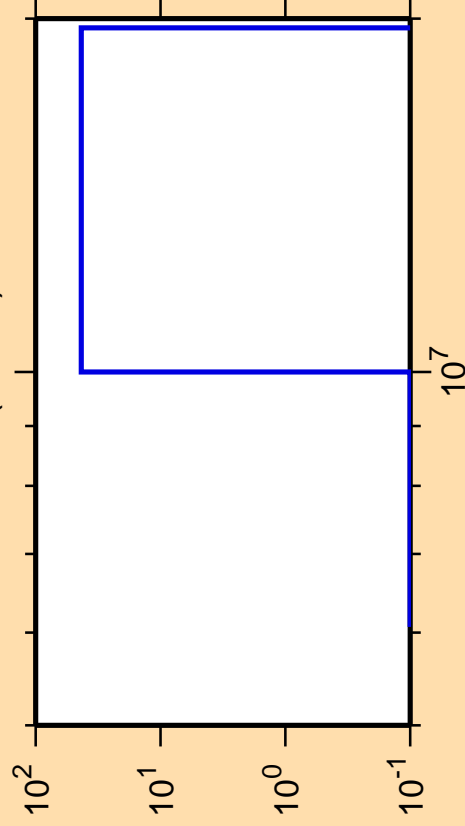
\Delta\sigma/\sigma vs. E for ^{68}\text{As} (mt 45)
