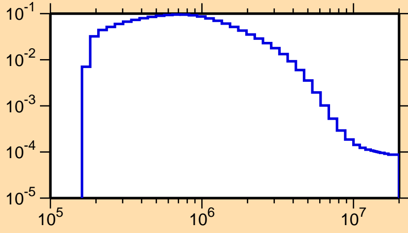
\sigma vs. E for ^{69}\text{As}(n,n_2)
