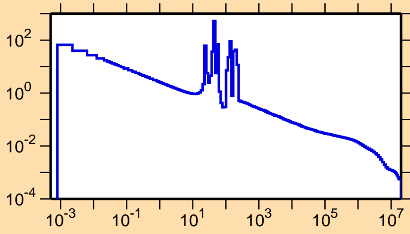
\sigma vs. E for ^{69}\text{As}(n,\gamma)
