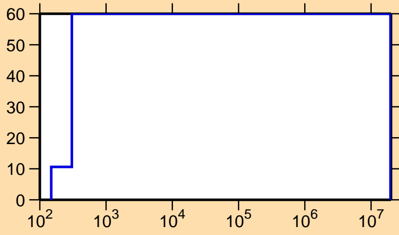
\Delta\sigma/\sigma vs. E for ^{69}\text{As}(n,\gamma)
