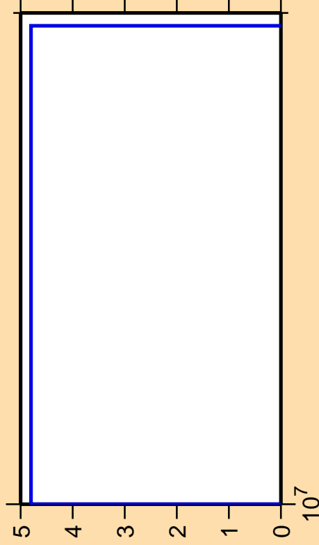
\Delta\sigma/\sigma vs. E for ^{69}\text{As} (mt 34)
