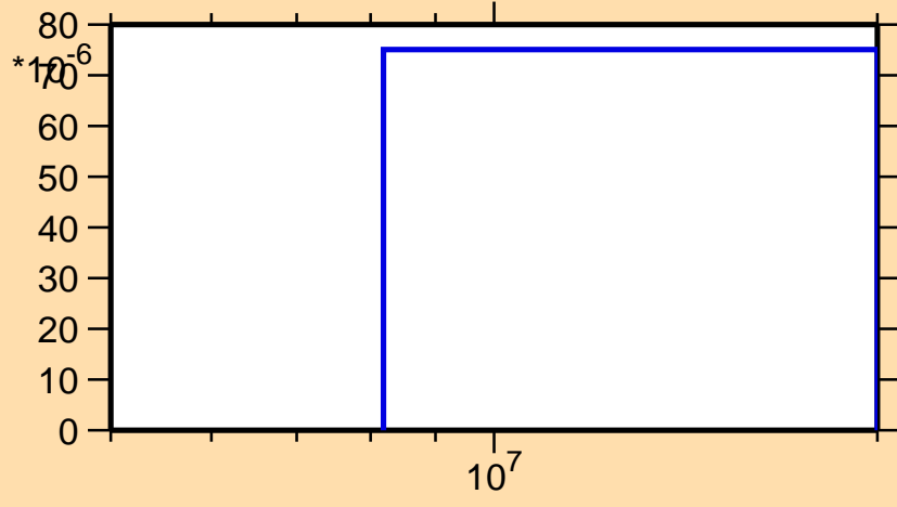
\sigma vs. E for ^{69}\text{As}(n,pd)
