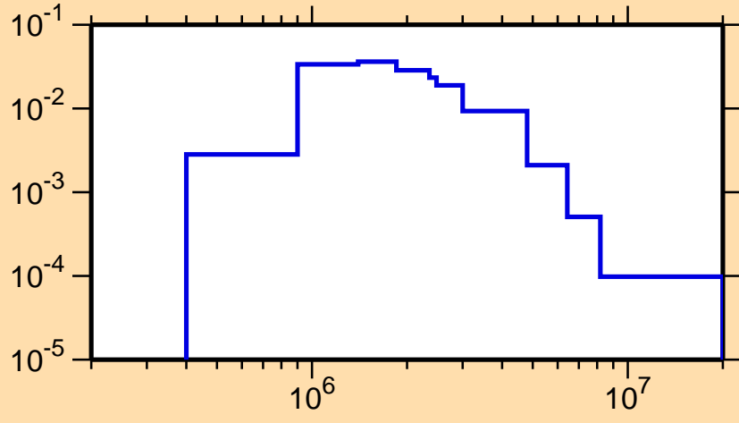
\sigma vs. E for ^{69}\text{As}(n,n_4)
