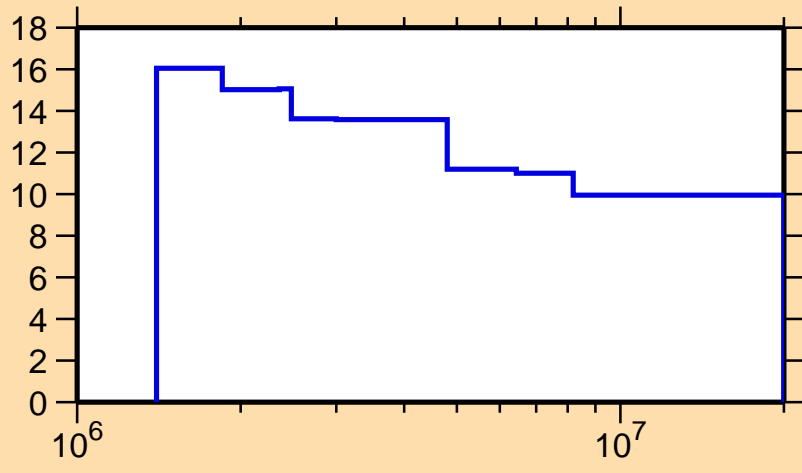
\Delta\sigma/\sigma vs. E for ^{69}\text{As}(n,n\text{onel.})
