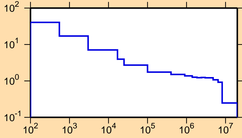
\sigma vs. E for ^{69}\text{As}(n,p)
