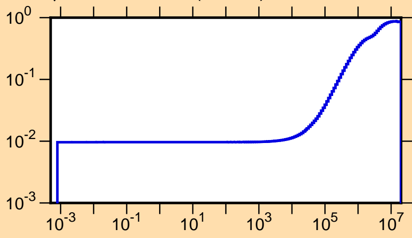
\mu vs. E for ^{70}\text{As}(\text{mt251})
