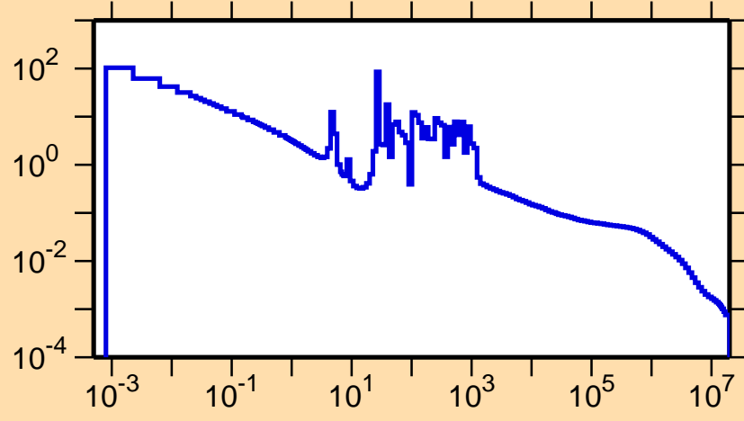
\sigma vs. E for ^{70}\text{As}(n,\gamma)
