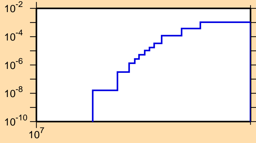
\sigma vs. E for ^{70}\text{As}(n,\text{nd})
