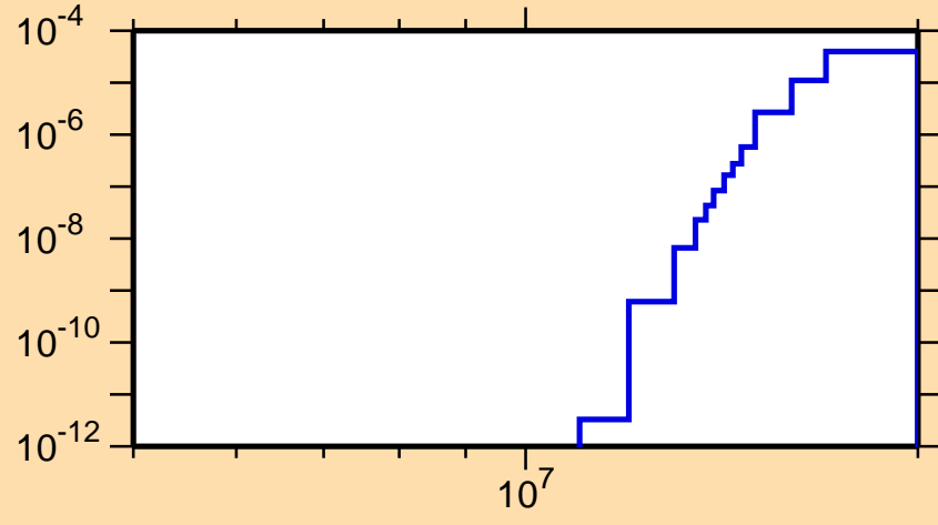
\sigma vs. E for ^{70}\text{As}(\text{mt117})
