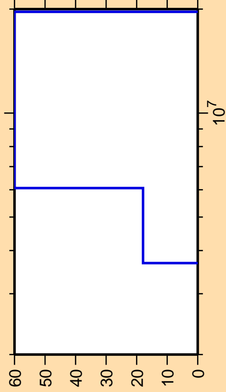
\Delta\sigma/\sigma vs. E for ^{70}\text{As}(n,n\alpha)
