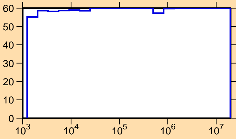
\Delta\sigma/\sigma vs. E for ^{70}\text{As}(n,\gamma)
