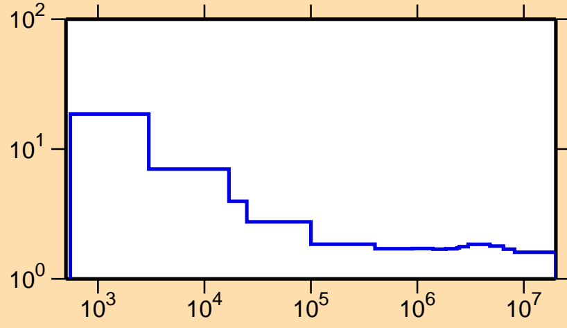
\sigma vs. E for ^{70}\text{As}(n,\text{nonel.})
