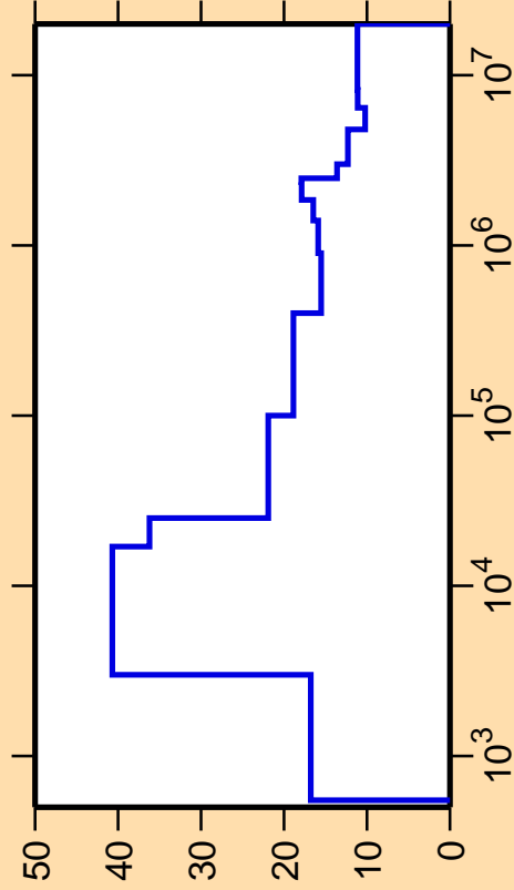
\Delta\sigma/\sigma vs. E for ^{70}\text{As}(n,\text{nonel.})
