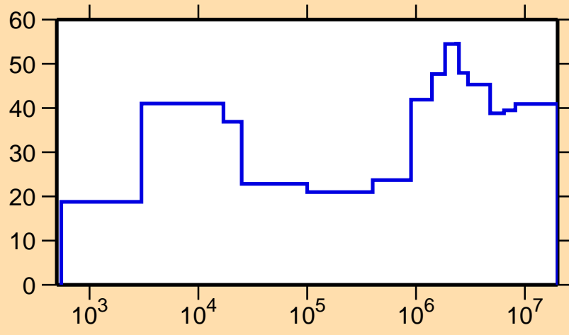
\Delta\sigma/\sigma vs. E for ^{70}\text{As}(n,p)
