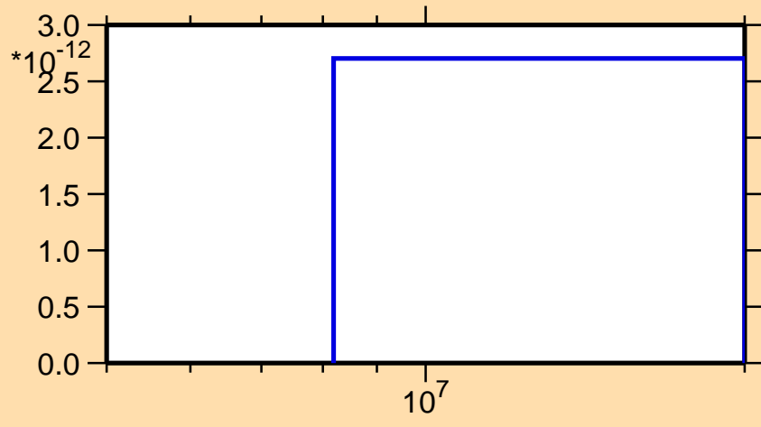
\sigma vs. E for ^{70}\text{As}(n,nt)
