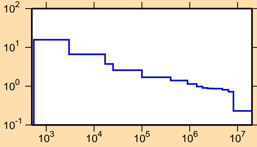
\sigma vs. E for ^{70}\text{As}(n,p)
