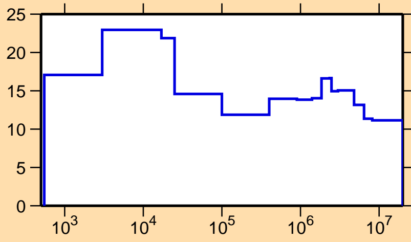
\Delta\sigma/\sigma vs. E for ^{70}\text{As}(n,el.)
