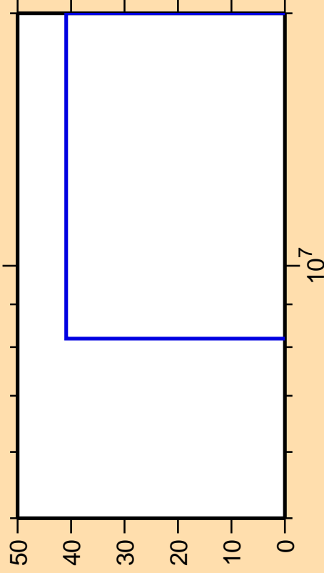
\Delta\sigma/\sigma vs. E for ^{70}\text{As}(n,p)
