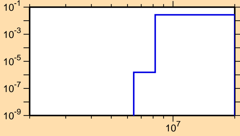
\sigma vs. E for ^{70}\text{As}(n,n\alpha)
