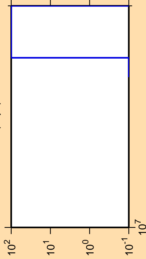
\Delta\sigma/\sigma vs. E for ^{71}\text{As}(n,pt)
