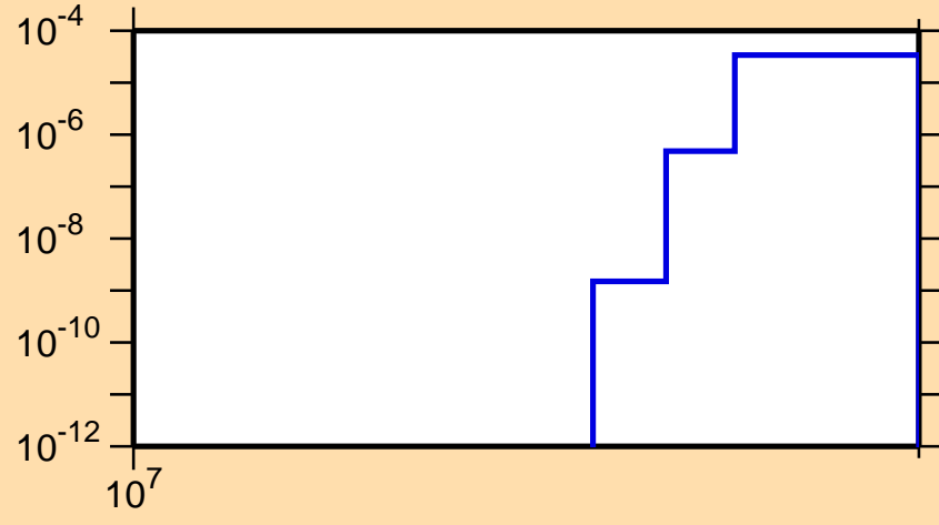
\sigma vs. E for ^{71}\text{As}(n,nd)
