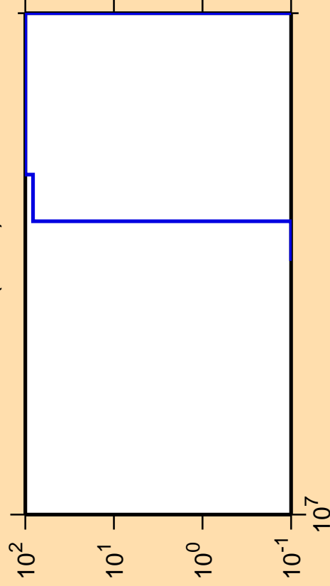
\Delta\sigma/\sigma vs. E for ^{71}\text{As}(n,nd)
