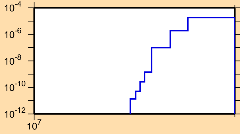
\sigma vs. E for ^{71}\text{As}(n,pd)
