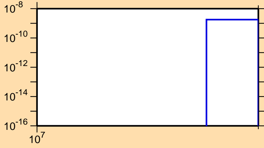
\sigma vs. E for ^{71}\text{As}(n,2n\alpha)
