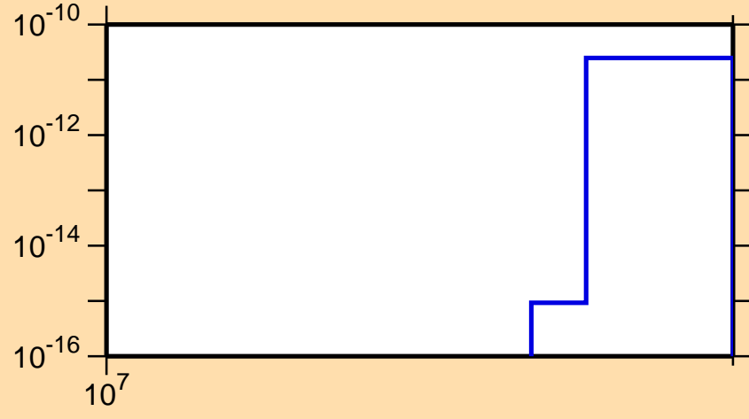
\sigma vs. E for ^{71}\text{As}(n,pt)
