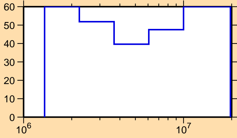
\Delta\sigma/\sigma vs. E for ^{71}\text{As}(n,n\text{cont.})
