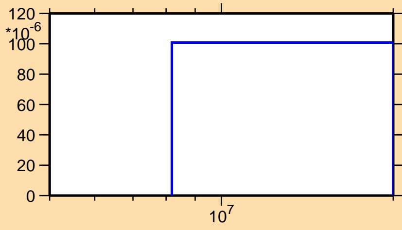
\sigma vs. E for ^{71}\text{As}(n,t)
