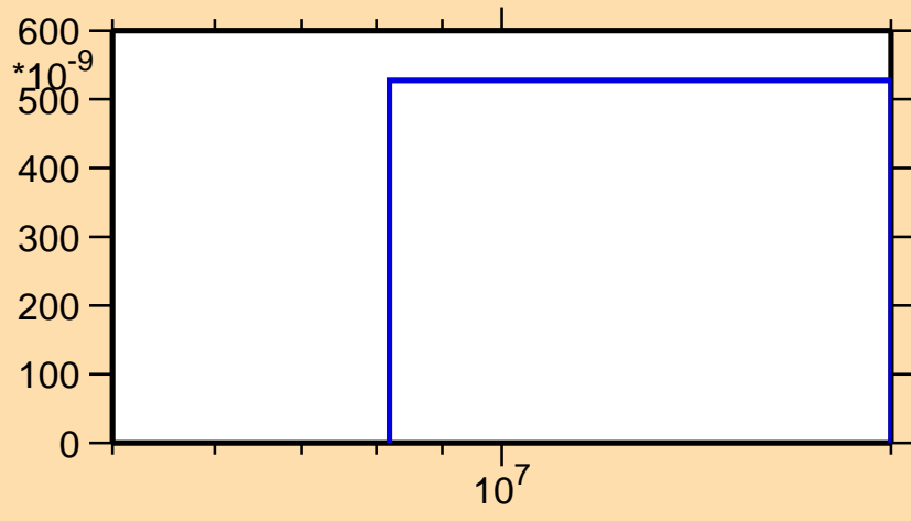
\sigma vs. E for ^{71}\text{As} (mt 45)
