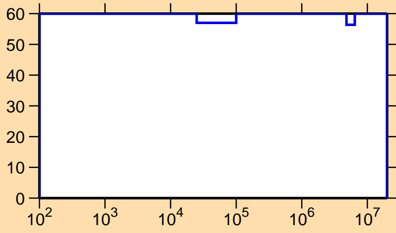
\Delta\sigma/\sigma vs. E for ^{71}\text{As}(n,\gamma)
