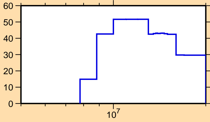
\Delta\sigma/\sigma vs. E for ^{72}\text{As}(n,\text{inel.})
