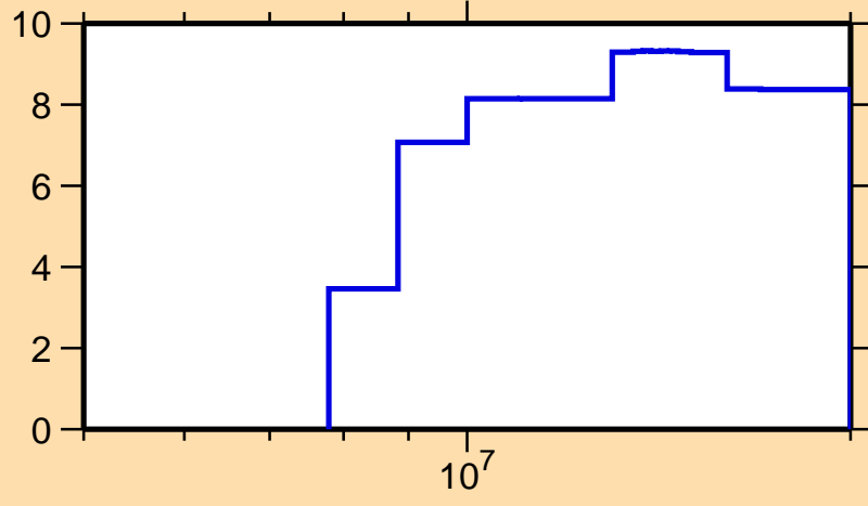
\Delta\sigma/\sigma vs. E for ^{72}\text{As}(n,\text{tot.})
