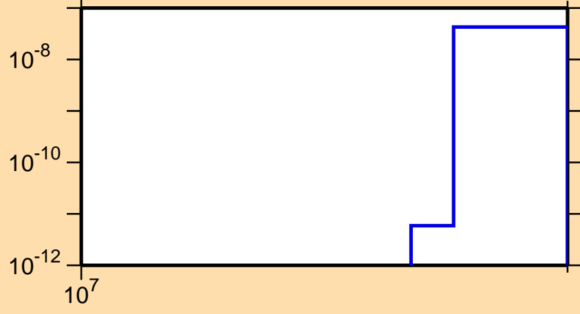
\sigma vs. E for ^{72}\text{As}(n,nt)
