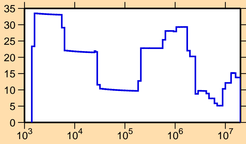
\Delta\sigma/\sigma vs. E for ^{72}\text{As}(n,el.)
