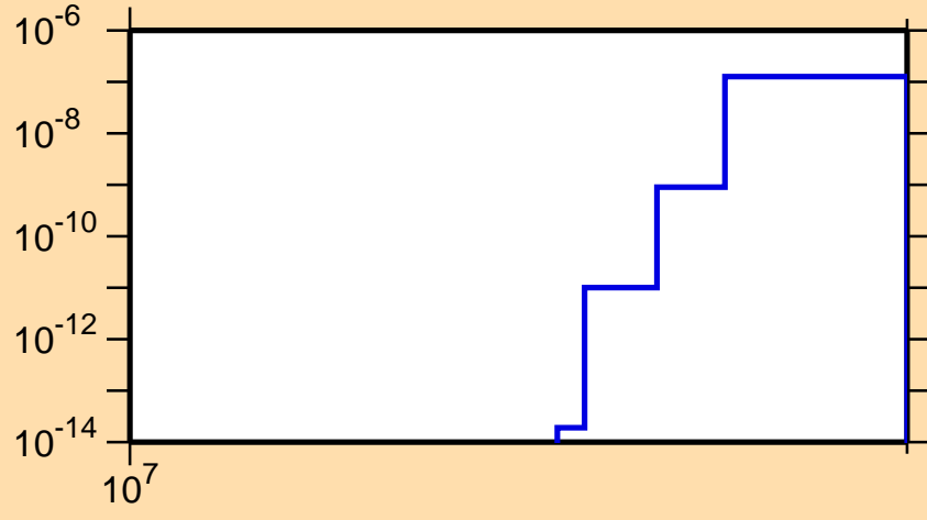
\sigma vs. E for ^{72}\text{As}(n,pd)
