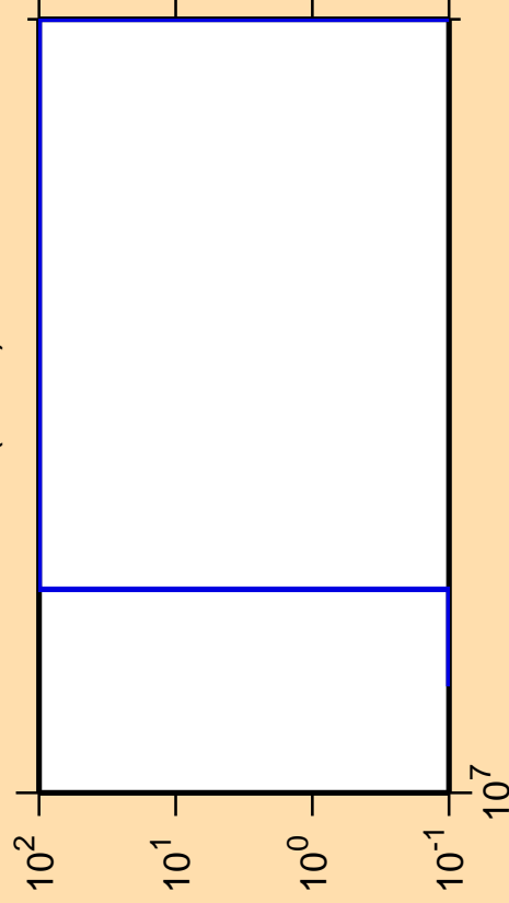
\Delta\sigma/\sigma vs. E for ^{72}\text{As}(n,nd)
