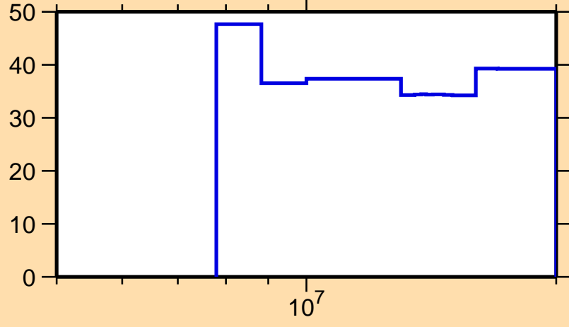
\Delta\sigma/\sigma vs. E for ^{72}\text{As}(n,2n)
