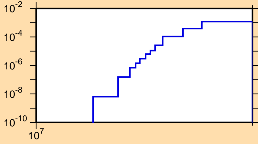
\sigma vs. E for ^{72}\text{As}(n,nd)
