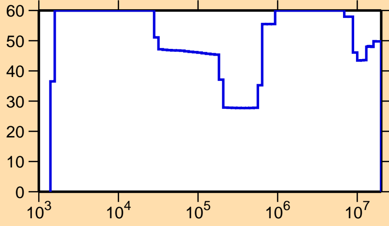
\Delta\sigma/\sigma vs. E for ^{72}\text{As}(n,p)
