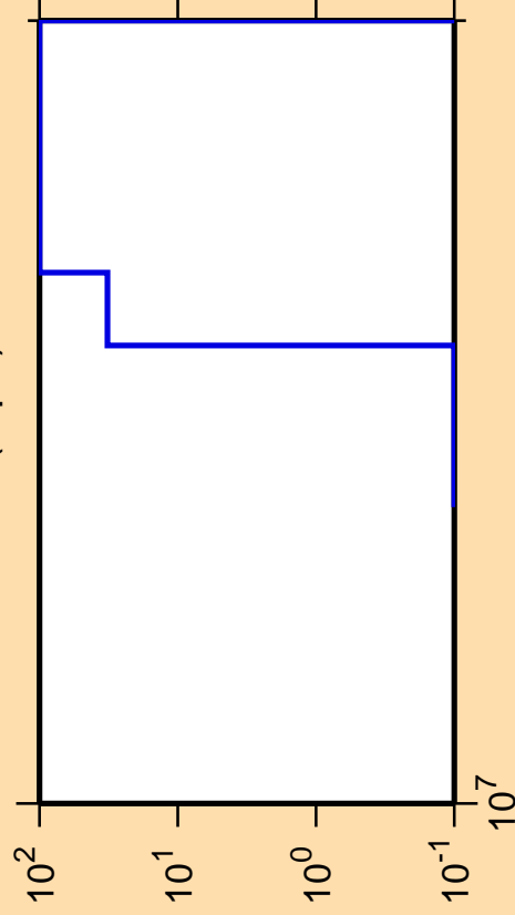
\Delta\sigma/\sigma vs. E for ^{72}\text{As}(n,pd)
