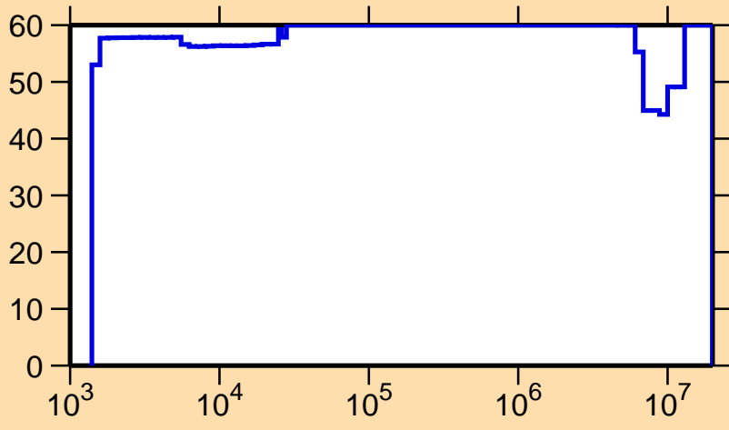
\Delta\sigma/\sigma vs. E for ^{72}\text{As}(n,\gamma)
