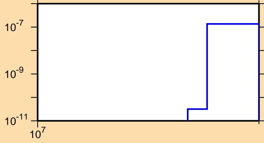
\sigma vs. E for ^{72}\text{As}(n,\text{pt})
