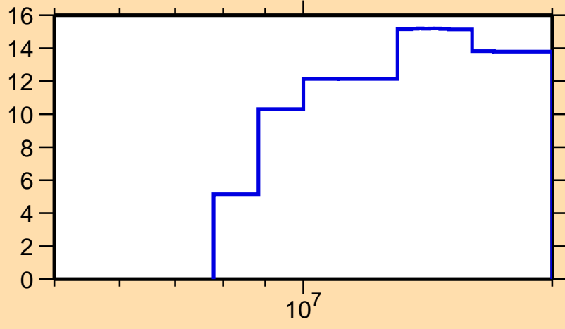
\Delta\sigma/\sigma vs. E for ^{72}\text{As}(n,\text{el.})
