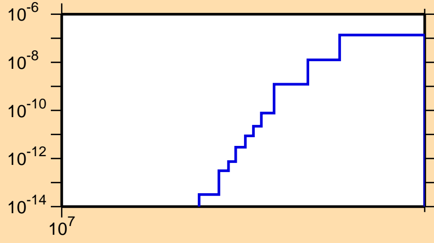
\sigma vs. E for ^{72}\text{As}(\text{mt117})
