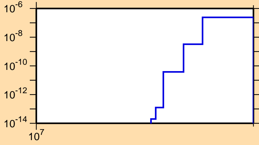
\sigma vs. E for ^{72}\text{As} (mt 45)
