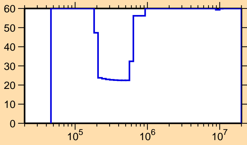
\Delta\sigma/\sigma vs. E for ^{72}\text{As}(n,n_1)
