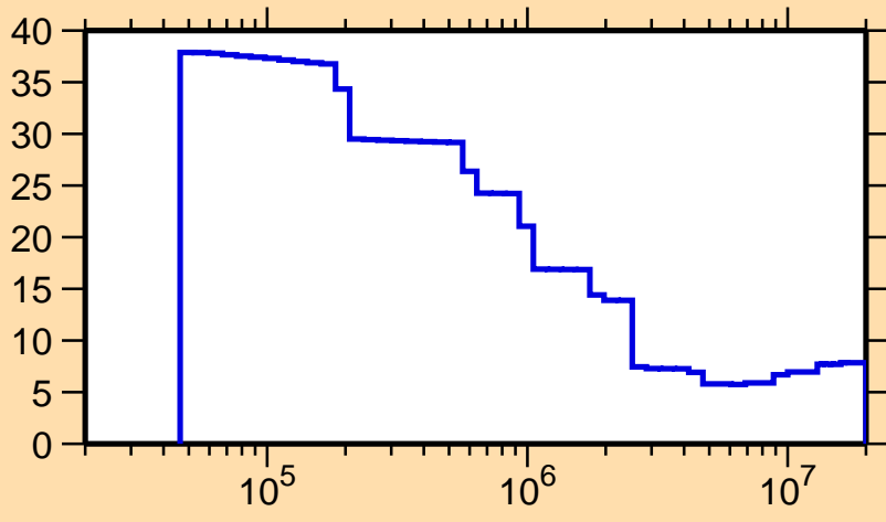
\Delta\sigma/\sigma vs. E for ^{72}\text{As}(n,\text{nonel.})
