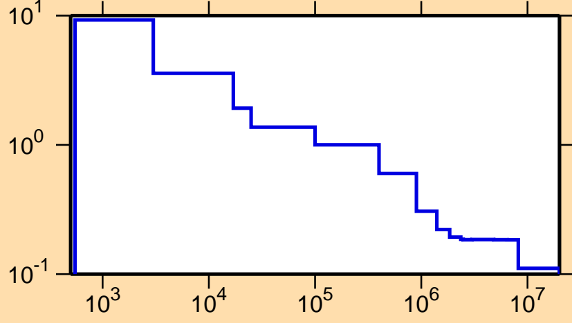
\sigma vs. E for ^{72}\text{As}(n,p)
