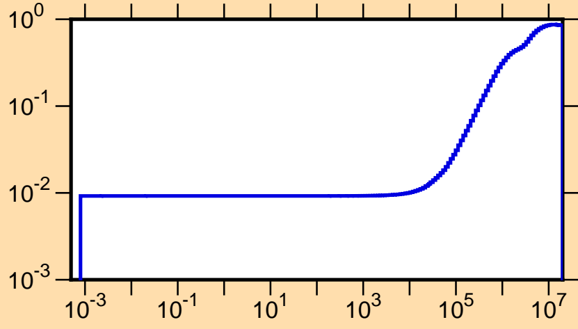
\mu vs. E for ^{73}\text{As}(\text{mt251})
