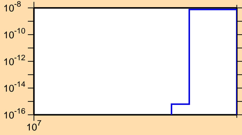
\sigma vs. E for ^{73}\text{As}(n,2n\alpha)
