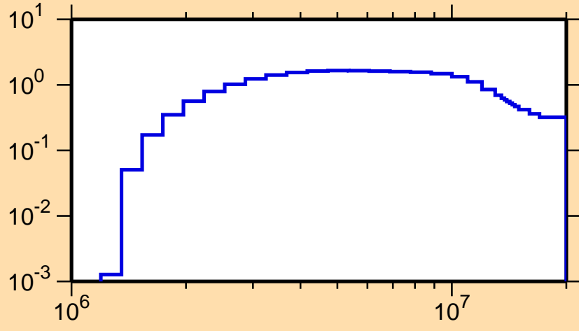
\sigma vs. E for ^{73}\text{As}(n,n\text{cont.})
