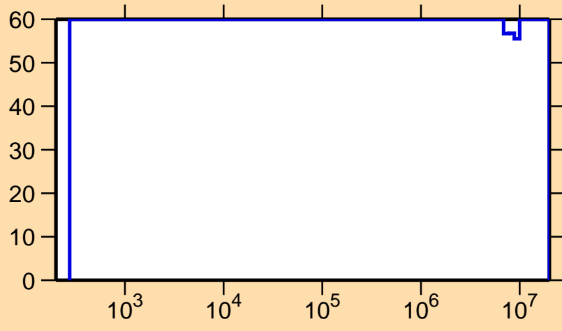
\Delta\sigma/\sigma vs. E for ^{73}\text{As}(n,\gamma)
