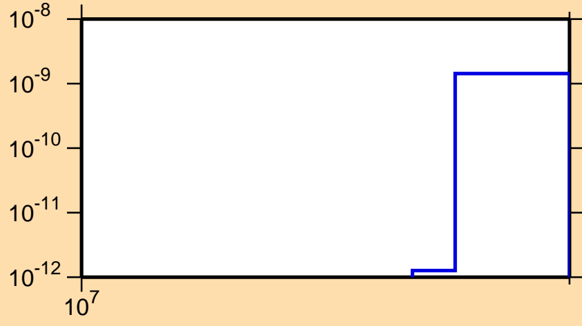
\sigma vs. E for ^{73}\text{As}(n,pd)
