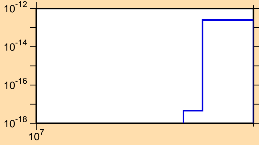
\sigma vs. E for ^{74}\text{As} (mt 34)
