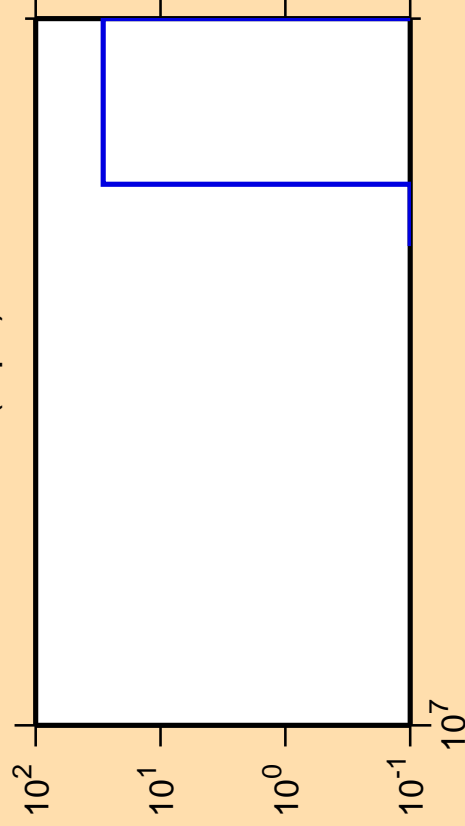
\Delta\sigma/\sigma vs. E for ^{74}\text{As}(n,pd)
