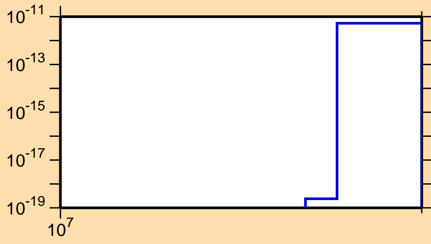
\sigma vs. E for ^{74}\text{As}(n,pd)
