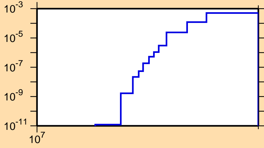
\sigma vs. E for ^{74}\text{As}(n,nd)
