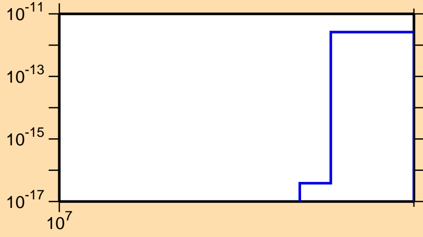
\sigma vs. E for ^{74}\text{As} (mt 45)
