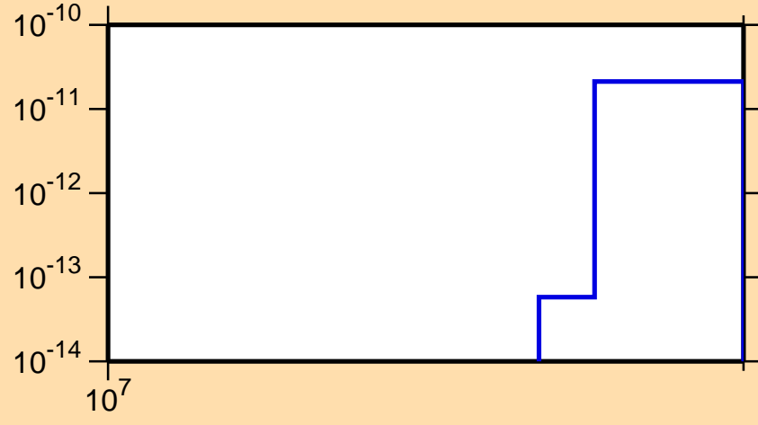
\sigma vs. E for ^{74}\text{As}(\text{mt117})
