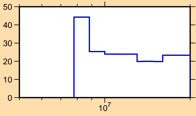
\Delta\sigma/\sigma vs. E for ^{74}\text{As}(n,2n)
