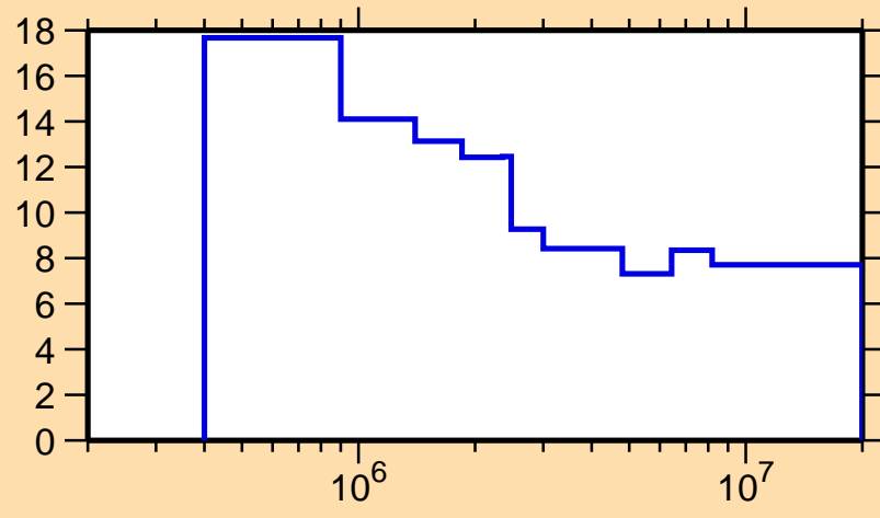
\Delta\sigma/\sigma vs. E for ^{74}\text{As}(n,n\text{onel.})
