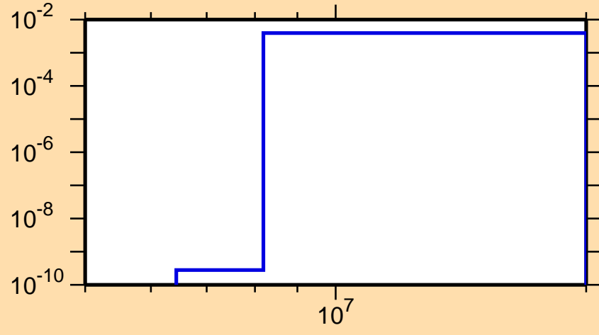
\sigma vs. E for ^{74}\text{As}(n,n\alpha)
