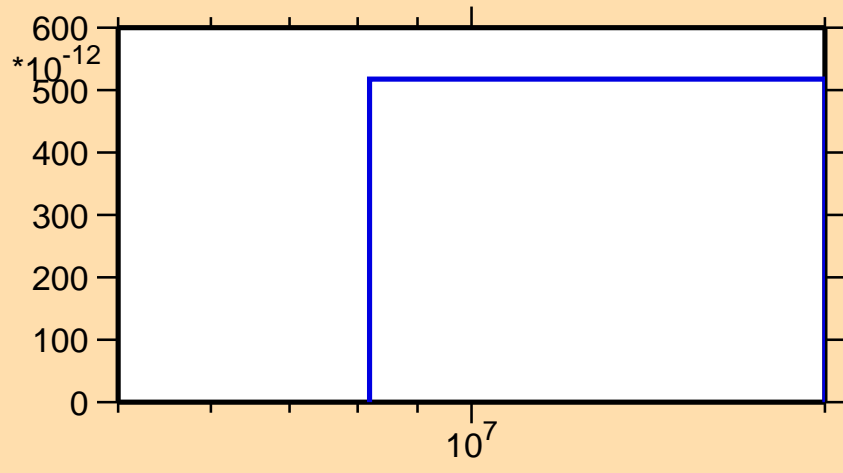
\sigma vs. E for ^{74}\text{As}(n,nt)
