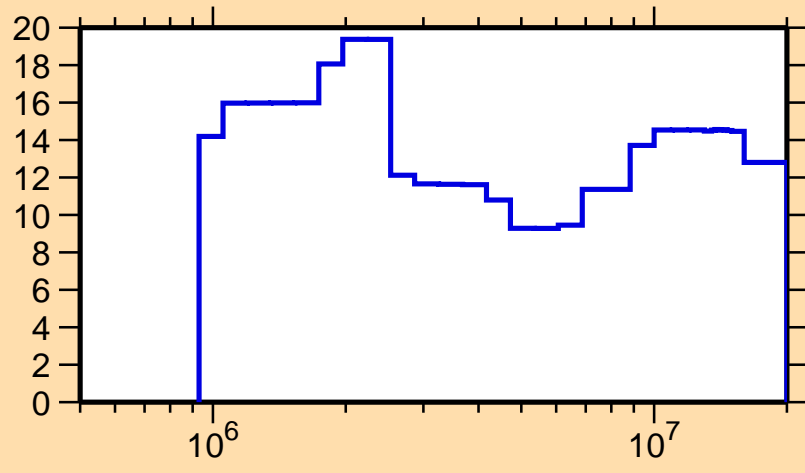
\Delta\sigma/\sigma vs. E for ^{75}\text{As}(n,el.)
