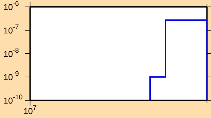
\sigma vs. E for ^{76}\text{As}(n,2n\alpha)
