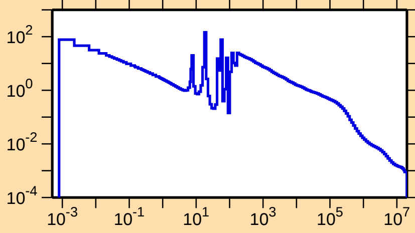
\sigma vs. E for ^{76}\text{As}(n,\gamma)
