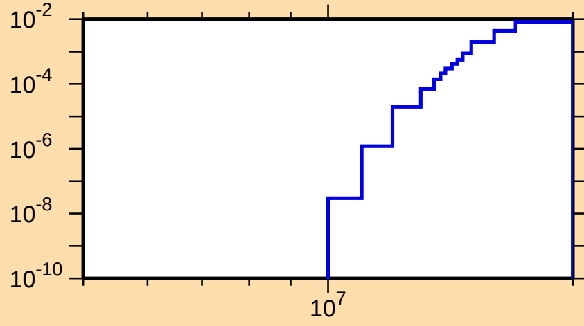
\sigma vs. E for ^{76}\text{As}(n,n\alpha)
