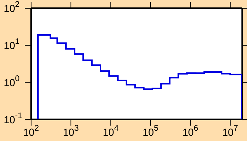
\sigma vs. E for ^{76}\text{As}(n,\text{nonel.})
