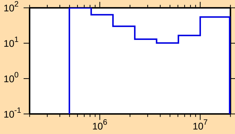
\Delta\sigma/\sigma vs. E for ^{76}\text{As}(n,n\text{cont.})
