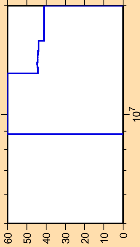
\Delta\sigma/\sigma vs. E for ^{77}\text{As}(n,p)
