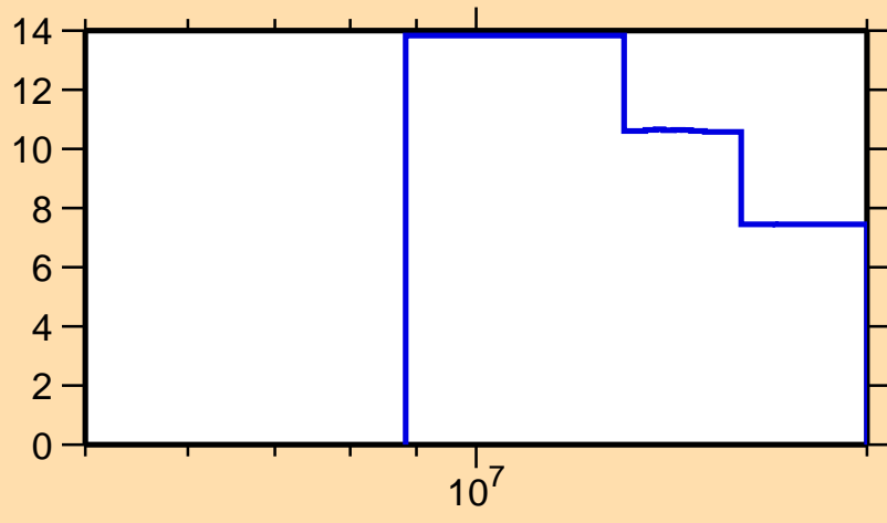
\Delta\sigma/\sigma vs. E for ^{77}\text{As}(n,2n)
