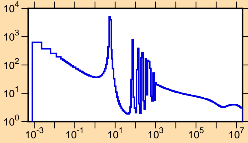
\sigma vs. E for ^{77}\text{As}(n,\text{tot.})
