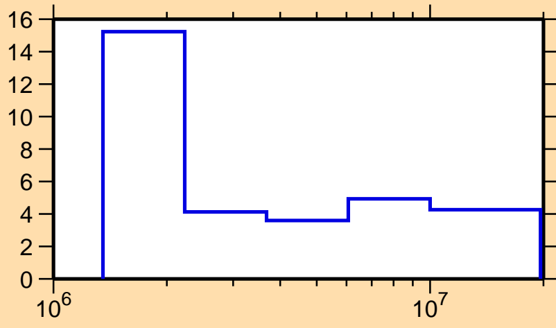
\Delta\sigma/\sigma vs. E for ^{77}\text{As}(n,n\text{onel.})
