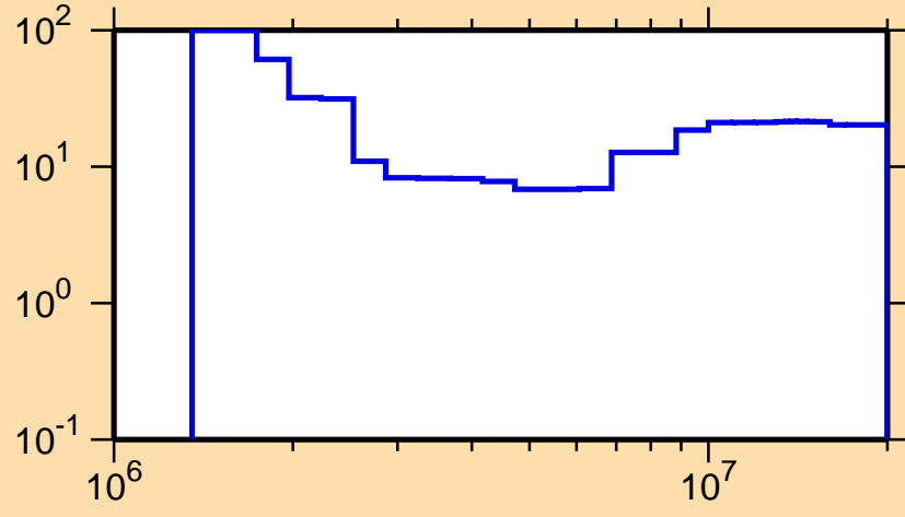
\Delta\sigma/\sigma vs. E for ^{78}\text{As}(n,ncont.)
