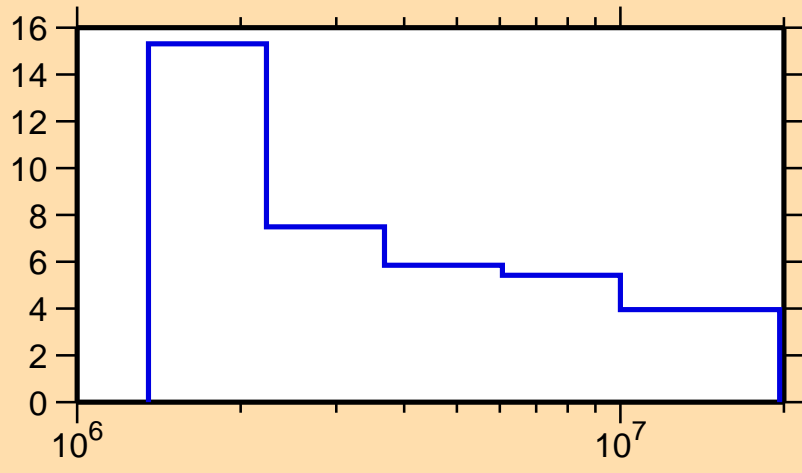
\Delta\sigma/\sigma vs. E for ^{78}\text{As}(n,n\text{onel.})
