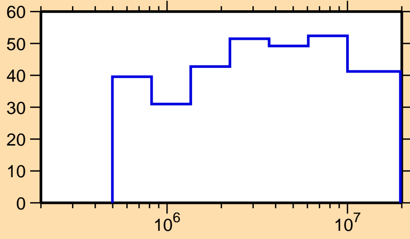
\Delta\sigma/\sigma vs. E for ^{78}\text{As}(n,\gamma)
