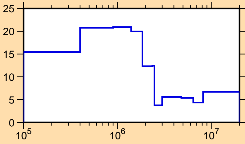
\Delta\sigma/\sigma vs. E for ^{78}\text{As}(n,\text{tot.})
