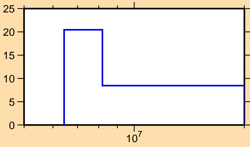
\Delta\sigma/\sigma vs. E for ^{78}\text{As}(n,2n)
