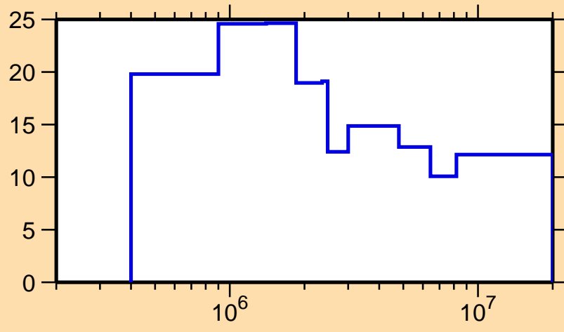
\Delta\sigma/\sigma vs. E for ^{78}\text{As}(n,el.)
