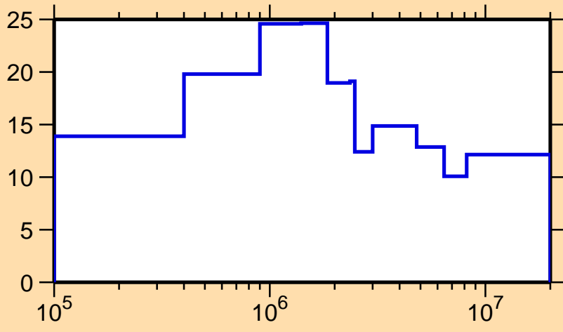
\Delta\sigma/\sigma vs. E for ^{78}\text{As}(n,\text{el.})
