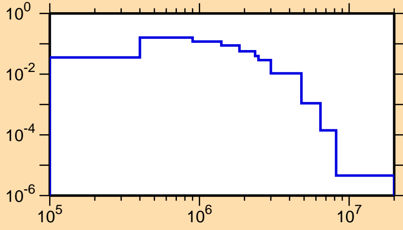
\sigma vs. E for ^{78}\text{As}(n,n_2)
