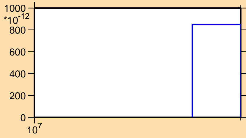
\sigma vs. E for ^{79}\text{As}(n,2np)
