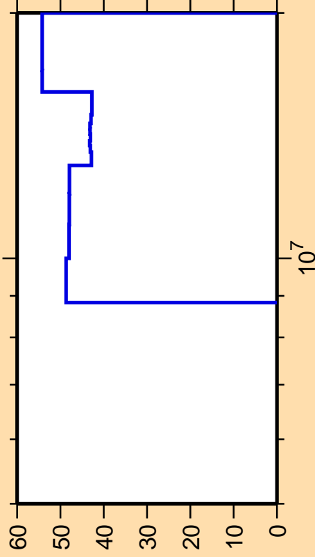
\Delta\sigma/\sigma vs. E for ^{79}\text{As}(n,\gamma)
