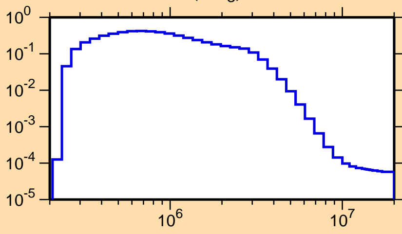
\sigma vs. E for ^{79}\text{As}(n,n_3)
