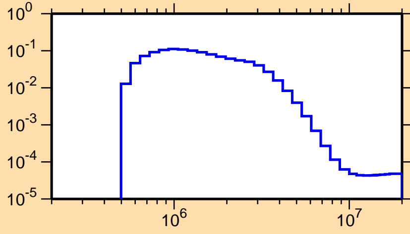
\sigma vs. E for ^{79}\text{As}(n,n_4)
