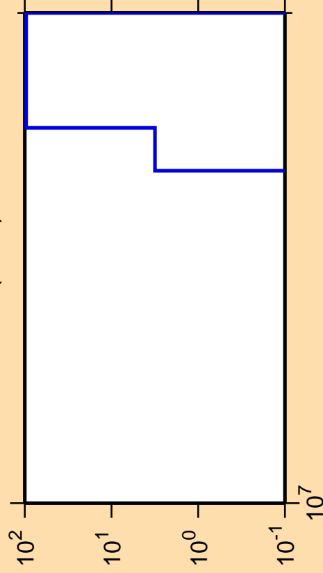
\Delta\sigma/\sigma vs. E for ^{79}\text{As}(n,nd)
