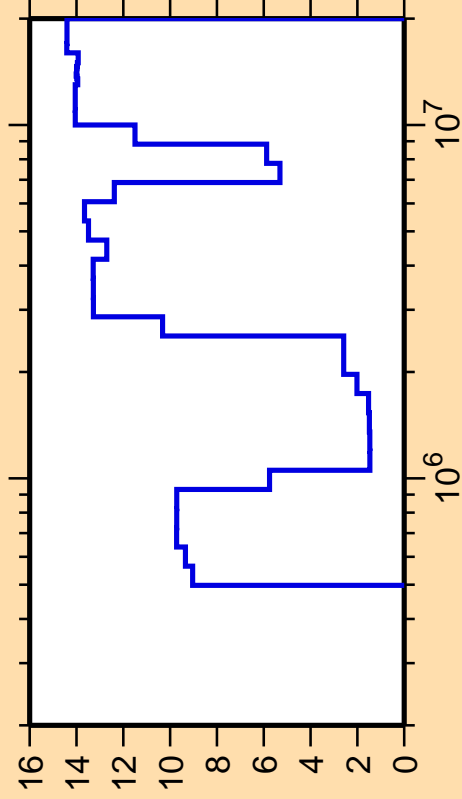
\Delta\sigma/\sigma vs. E for ^{79}\text{As}(n,n_4)
