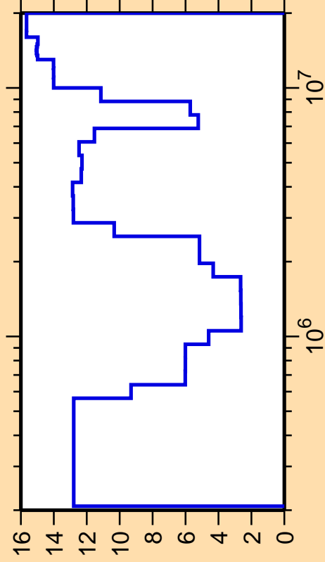
\Delta\sigma/\sigma vs. E for ^{79}\text{As}(n,n_3)
