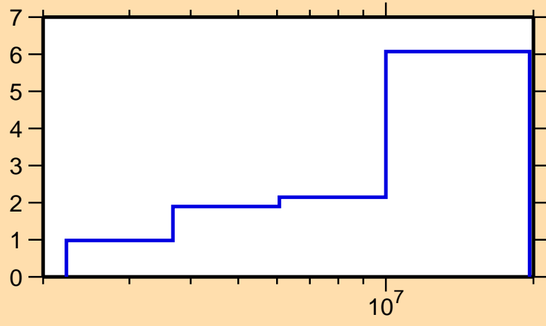
\Delta\sigma/\sigma vs. E for ^{79}\text{As}(n,el.)
