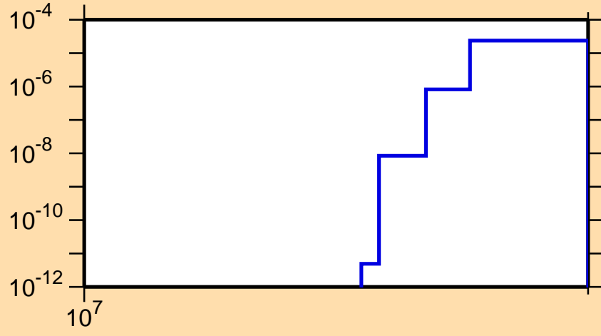
\sigma vs. E for ^{80}\text{As}(n,nd)
