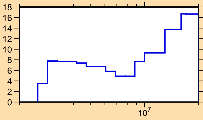
\Delta\sigma/\sigma vs. E for ^{80}\text{As}(n,\text{tot.})
