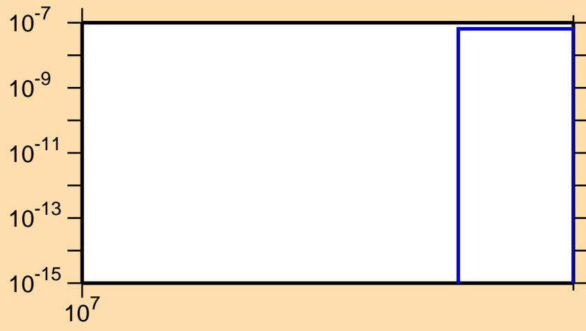
\sigma vs. E for ^{80}\text{As}(n,nt)
