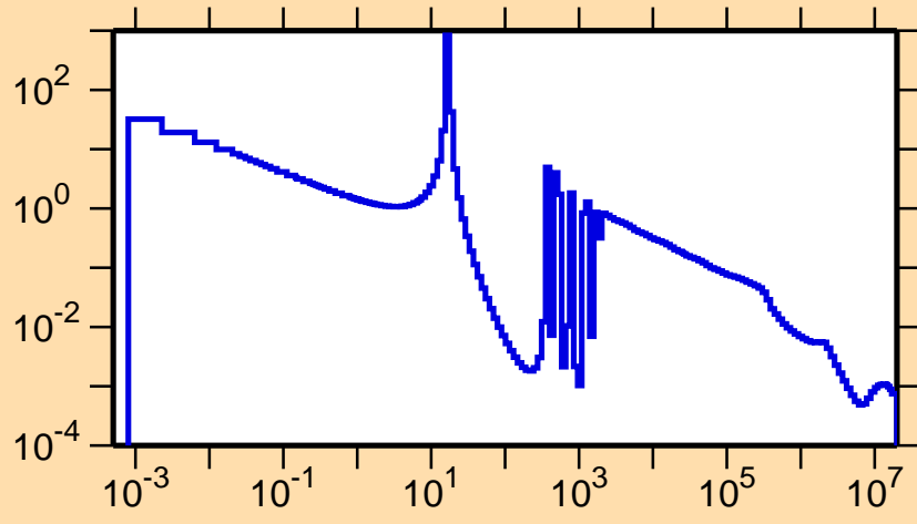
\sigma vs. E for ^{80}\text{As}(n,\gamma)
