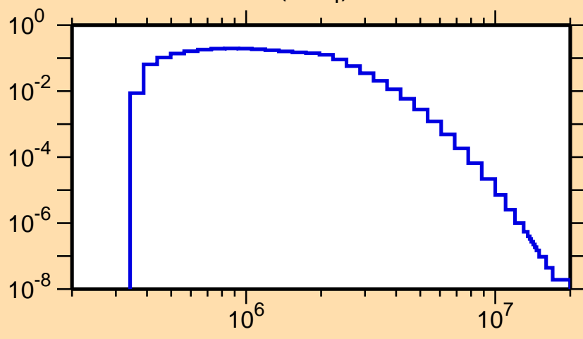
\sigma vs. E for ^{80}\text{As}(n,n_4)
