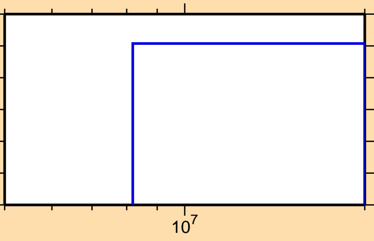
\sigma vs. E for ^{80}\text{As}(n,t)
